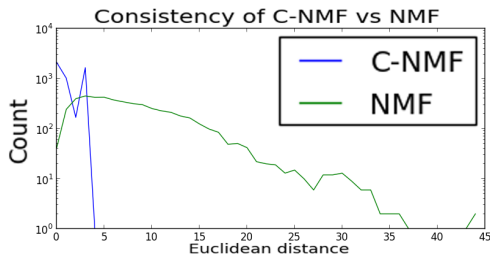
Fig. 3. Logarithmic histogram of distances between 100 sets of decomposition matrices obtained with C-NMF (blue) and NMF (green) from the song Help! by The Beatles.
