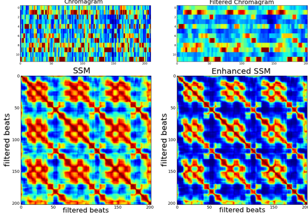
Fig. 1. Example of a chromagram (top-left), a pre-filtered chromagram with h = 9 (top-right), an original SSM using the correlation distance (bottom-left), and an enhanced SSM (bottom-right), of the song Help! by The Beatles.
