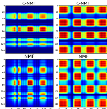
Fig. 2. Decomposition matrices of C-NMF (top) and NMF (bottom) with a rank of decomposition of r = 2 from the song Tell Me Why by The Beatles.
