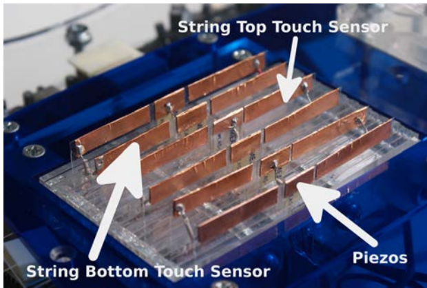
Figure 3. The plucking system of the BLADEAXE. We can see the three bands of copper tape on each "string" used to detect the plucking position and to minimize the impact of electromagnetic fields on the piezoelectric films signal.
