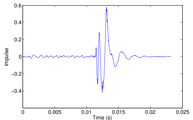
Figure 4. Waveform of a pulse created on one the polycarbonate sheet of the BLADEAXE plucking system. The pluck was carried out on the upper side of the sheet with the skin of the thumb.
