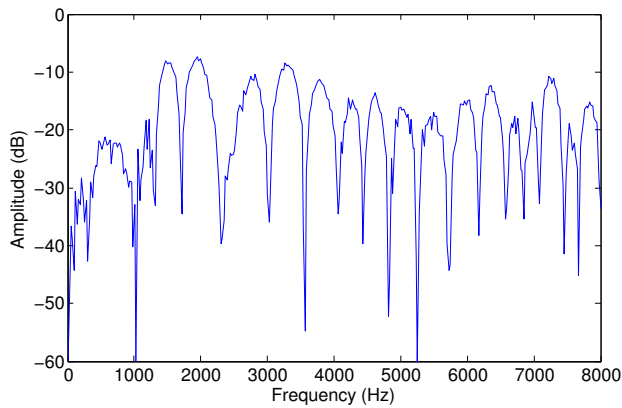
Figure 5. Fast Fourier Transform of the signal of the pulse presented in figure 4.
