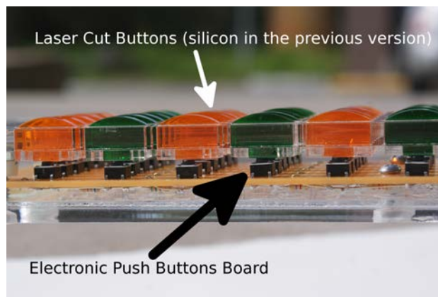
Figure 10. Electronic push-buttons fret board with laser-cut acrylic buttons over them as they appear in the final version of the BLADEAXE neck. The same electronic push-buttons fret board was used for the silicon and the first laser-cut acrylic buttons versions of the neck.
