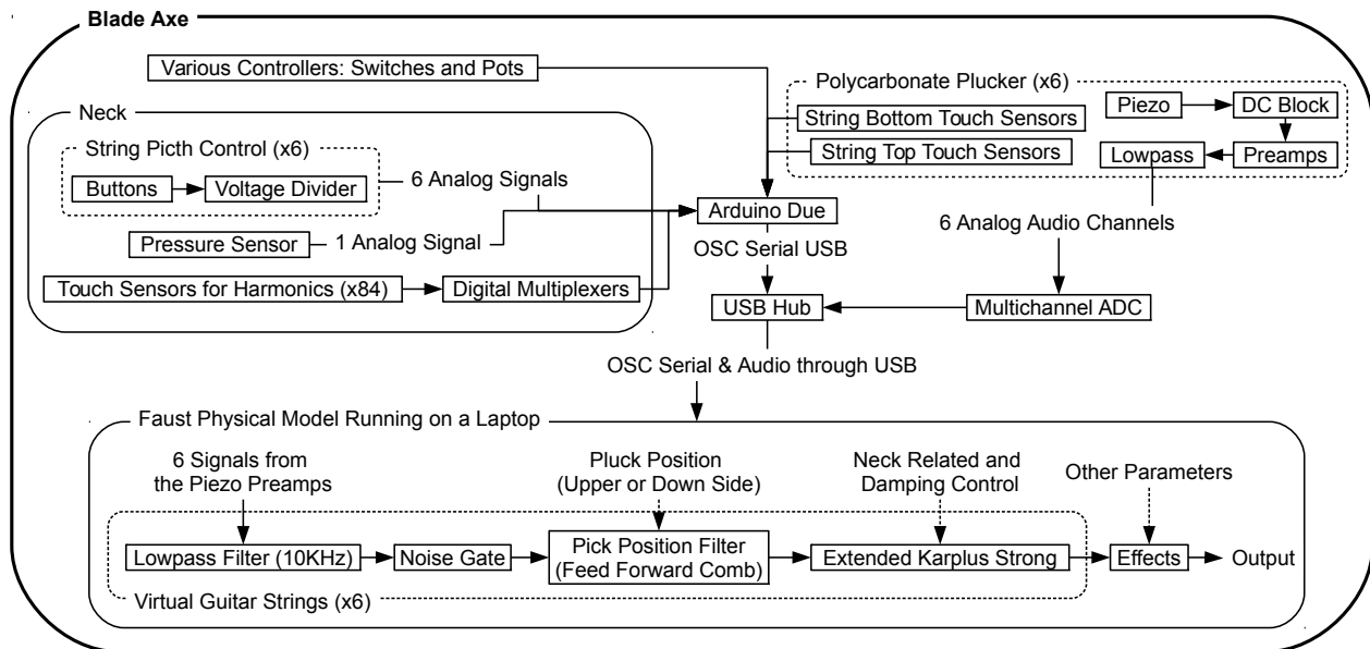
Figure 1. Overview of the different components of the BLADEAXE.
