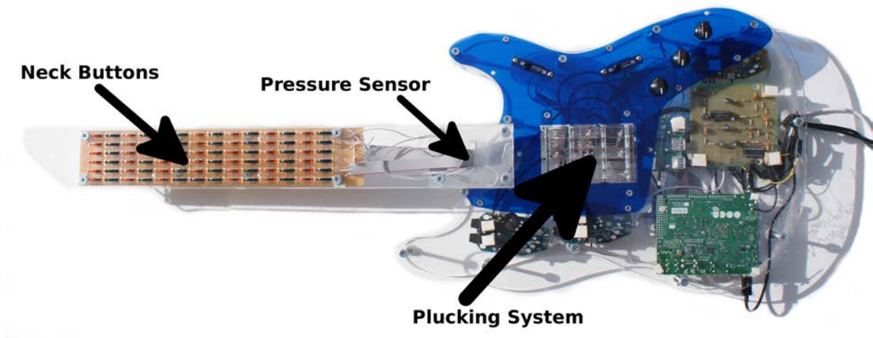
Figure 2. Top view of the BLADEAXE.
