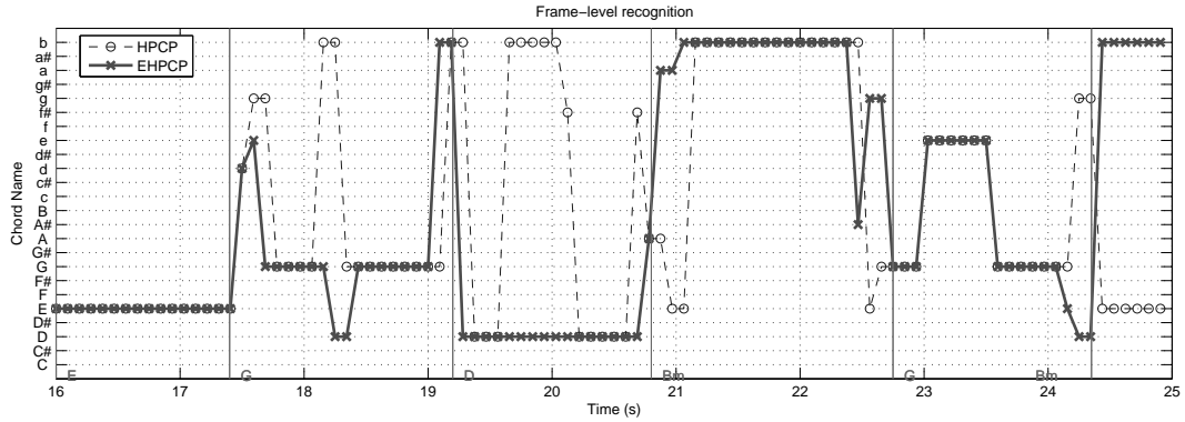
Figure 7: Frame-level chord recognition results of an excerpt from The Beatles Eight Days a Week . Vertical lines denote manually annotated chord boundaries with chord names.
