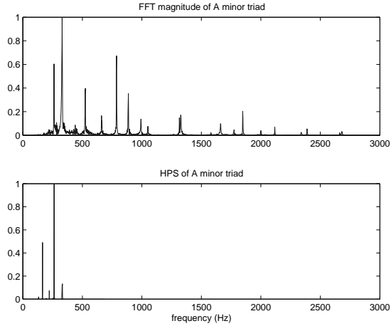
Figure 3: DFT of A minor triad example (above) and its Harmonic Product Spectrum (below)
