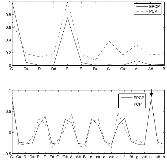
Figure 4: EPCP vector of an A minor triad, and its correlation with 24 major/minor triad templates. Arrow in the lower figure represents the maximum correlation.
