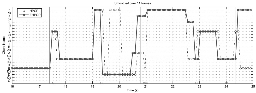
Figure 8: Chord recognition results after a smoothing process across 11 frames of an excerpt from The Beatles Eight Days a Week . Vertical lines denote manually annotated chord boundaries with chord names.
