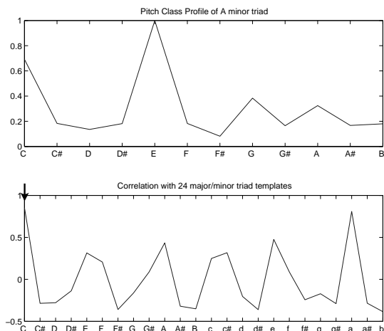
Figure 2: Chroma vector of an A minor triad, and its correlation with 24 major/minor triad templates. Arrow in the lower figure denotes where the maximum correlation occurs.
