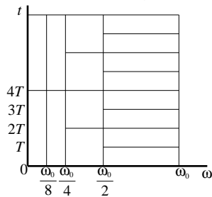
(Dyadic) Discrete Wavelet Transform Tiling
