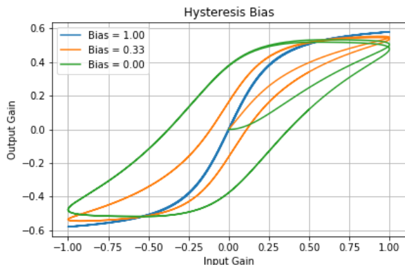
Figure 6: Hysteresis curves with varying bias
