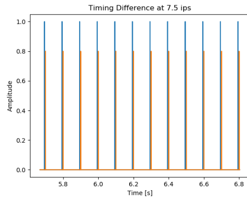
Figure 4: Input pulse train superimposed with pulse train recorded from TC-260
