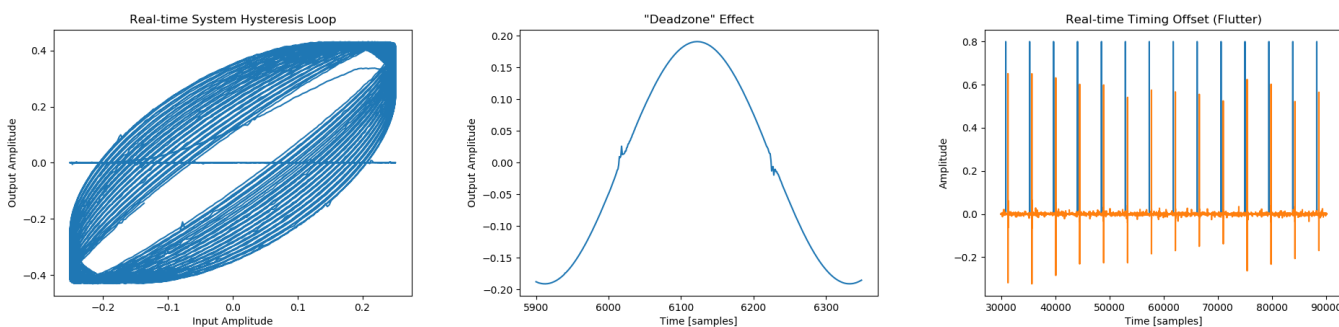
Figure 6: Testing results for real-time system: input vs. output amplitude for variable frequency sine wave (left), sine wave output with no biasing (center), input vs. output pulse train comparison (right).
