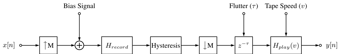
Figure 5: Flowchart of real-time system: M is the oversampling factor, H_{record} is the transfer function of the record head, and H_{play} is the play head transfer function including loss effects, and a de-biasing filter.
