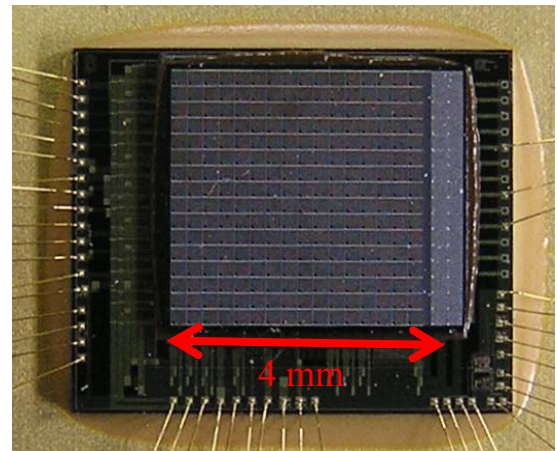
Figure 4. CMUT array flip-chip bonded to an integrated circuit that comprises the front-end circuitry for the array.
