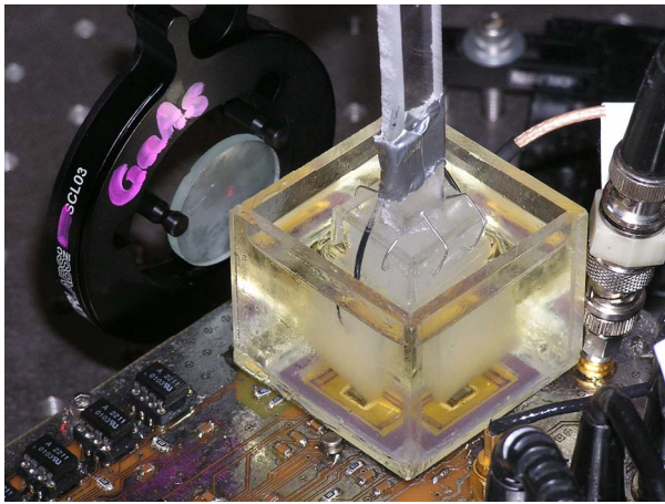
Figure 2. Photograph of the phantom and tank. The transducer array is located at the bottom of the tank. The diffuser at the left diffuses the laser beam to provide more uniform illumination of the sample.
