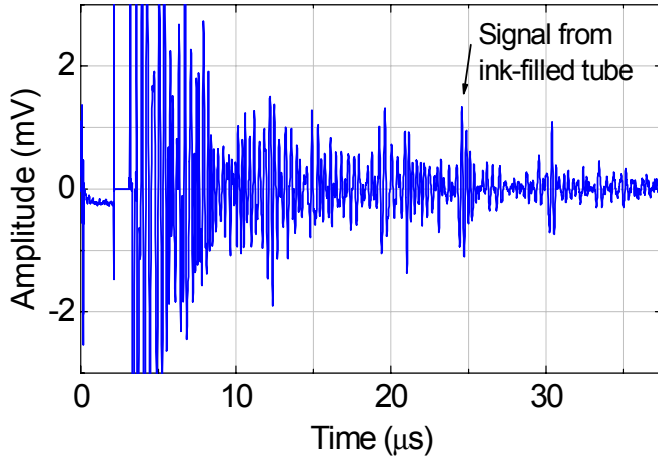
Figure 6. Example pulse-echo A-scan. Reflections from the three tubes can be identified.
