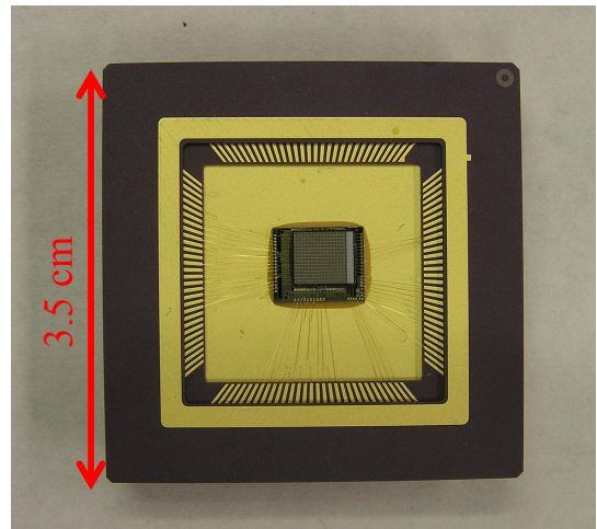
Figure 3. Package containing the transducer array and electronics.
