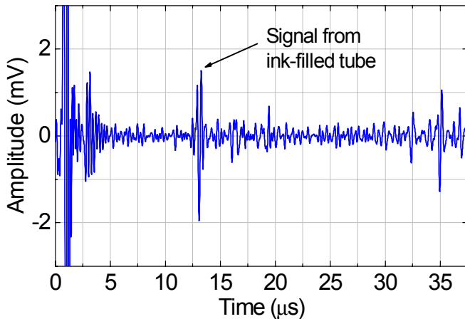
Figure 7. Photoacoustic data acquired for a single element. The signal from the ink-filled tube can be clearly seen. The signals seen in the first 5- \mu s are due to electronic noise of the laser and laser light incident on the transducer array.
