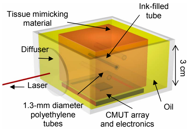
Figure 1. Vessel-like photoacoustic imaging phantom. Three 1.3-mm diameter tubes are inside a block of tissue mimicking material. The center tube is filled with ink to provide optical contrast. The phantom is illuminated by a laser from the side.
