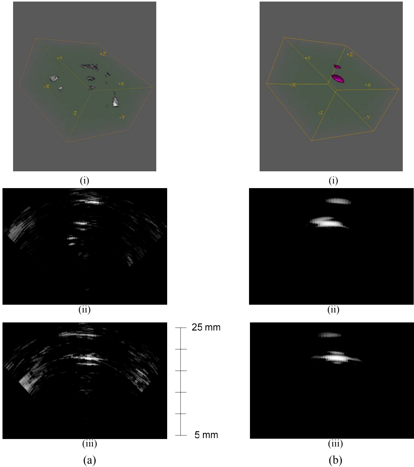
Figure 5. (a) Pulse-echo images of the phantom shown with 30-dB dynamic range. (b) Photoacoustic images shown with 20-dB dynamic range. The volume rendered image is shown in (i). XZ and YZ cross sections are shown in (ii) and (iii) respectively.
