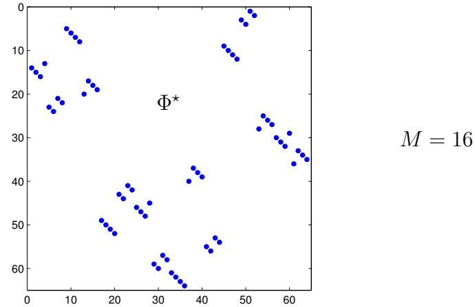
Figure 117: Sparsity pattern for composite permutation matrix \Phi^* \in \mathbb{R}^{4M \times 4M} representing solution from Figure 112b. Each four-point cluster represents a circulant permutation matrix from (867). Any M=16 -piece solution may be verified on the TOMY website .
