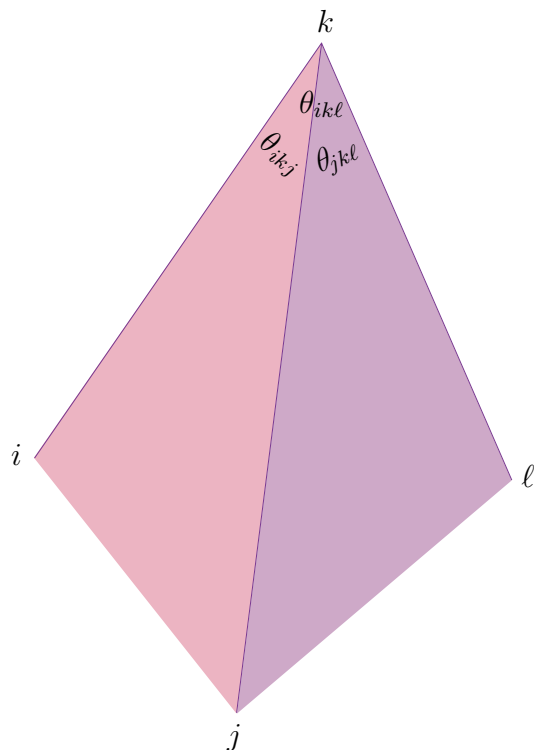
Figure 123: Fifth Euclidean metric property nomenclature. Each angle \theta is made by a vector pair at vertex k while i, j, k, l index four points at the vertices of a generally irregular tetrahedron. The fifth property is necessary for realization of four or more points; a reckoning by three angles in any dimension. Together with the first four Euclidean metric properties, this fifth property is necessary and sufficient for realization of four points.
