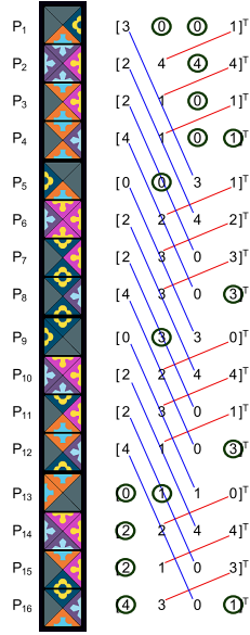
Figure 116: \circ indicate boundary \beta , line segments indicate differences \Delta . Entries are indices \ell to standard basis vectors e_\ell \in \mathbb{R}^L from Figure 115.
