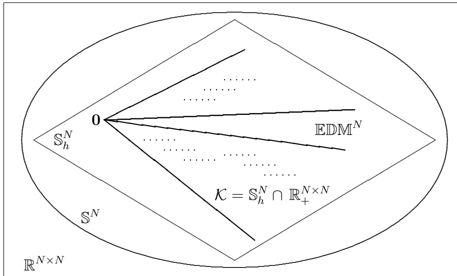
Figure 158: Pseudo-Venn diagram: The EDM cone belongs to the intersection of the symmetric hollow subspace with the nonnegative orthant; \text{EDM}^N \subseteq \mathcal{K} (922). \text{EDM}^N cannot exist outside \mathbb{S}_h^N , but \mathbb{R}_+^{N \times N} does.
