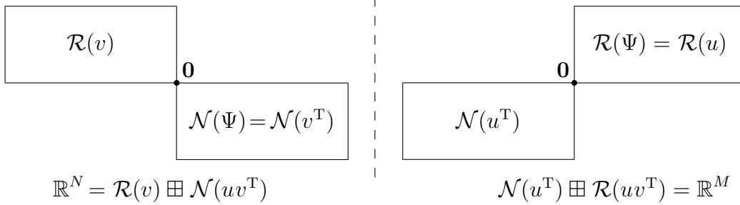
Figure 162: The four fundamental subspaces [334, §3.6] of any dyad \Psi = uv^T \in \mathbb{R}^{M \times N} : \mathcal{R}(v) \perp \mathcal{N}(\Psi) & \mathcal{N}(u^T) \perp \mathcal{R}(\Psi) . \Psi(x) \triangleq uv^T x is a linear mapping from \mathbb{R}^N to \mathbb{R}^M . Map from \mathcal{R}(v) to \mathcal{R}(u) is bijective. [332, §3.1]
