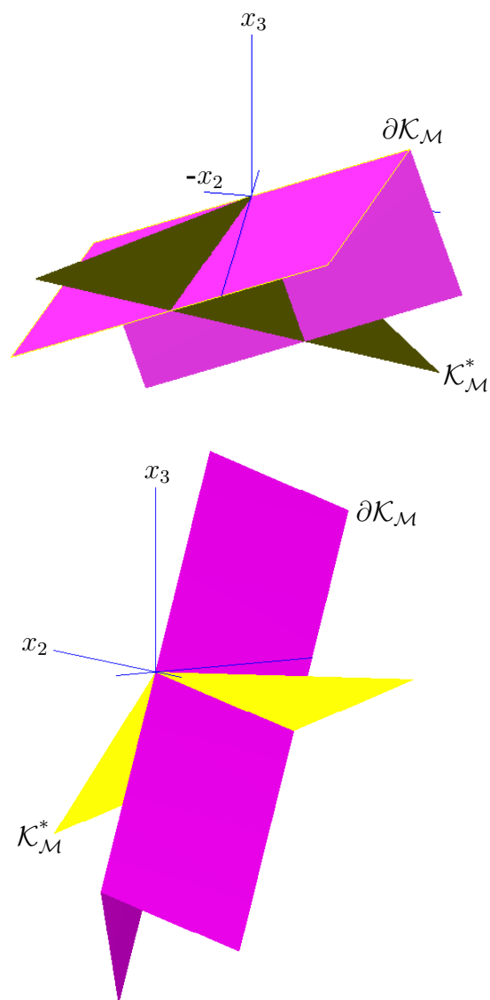
Figure 66: Two views of monotone cone \mathcal{K}_M and its dual \mathcal{K}_M^* (drawn truncated) in \mathbb{R}^3 . Monotone cone is not pointed. Dual monotone cone is not full-dimensional. Cartesian coordinate axes are drawn for reference.
