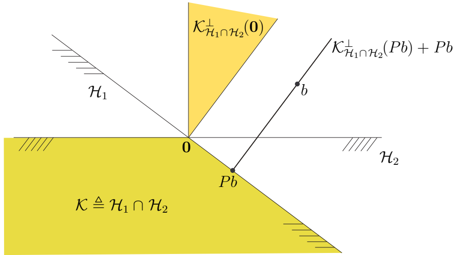
Figure 181: Two examples (truncated): normal cone to \mathcal{H}_1 \cap \mathcal{H}_2 at the origin and at point Pb on the boundary. \mathcal{H}_1 and \mathcal{H}_2 are the same halfspaces from Figure 180. Normal cone at the origin \mathcal{K}_{\mathcal{H}_1 \cap \mathcal{H}_2}^\perp(\mathbf{0}) is simply -\mathcal{K}^* .
