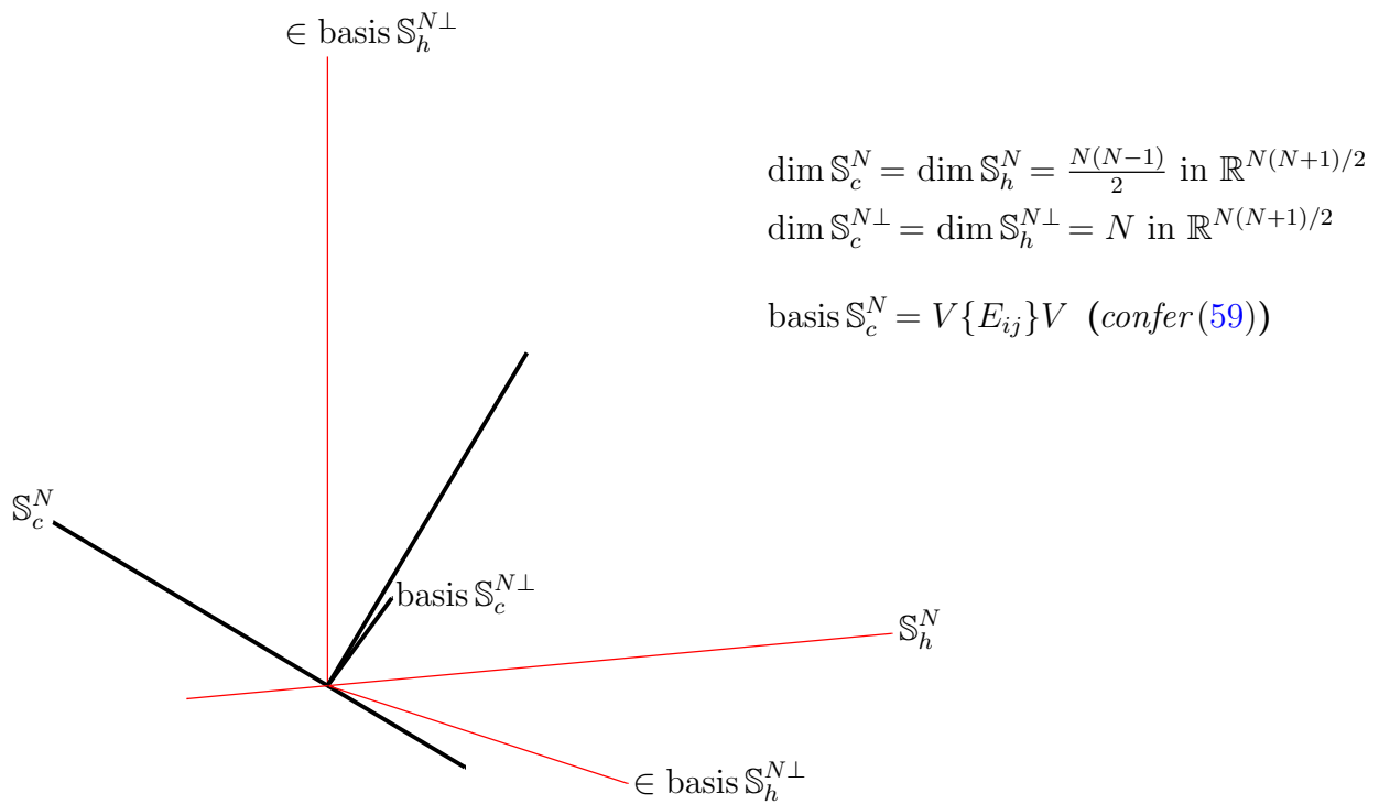
Figure 135: Orthogonal complements in \mathbb{S}^N abstractly oriented in isometrically isomorphic \mathbb{R}^{N(N+1)/2} . Case N = 2 accurately illustrated in \mathbb{R}^3 . Orthogonal projection of basis for \mathbb{S}_h^{N\perp} on \mathbb{S}_c^{N\perp} yields another basis for \mathbb{S}_c^{N\perp} . (Basis vectors for \mathbb{S}_c^{N\perp} are illustrated lying in a plane orthogonal to \mathbb{S}_c^N in this dimension. Basis vectors for each \perp space outnumber those for its respective orthogonal complement; such is not the case in higher dimension.)
