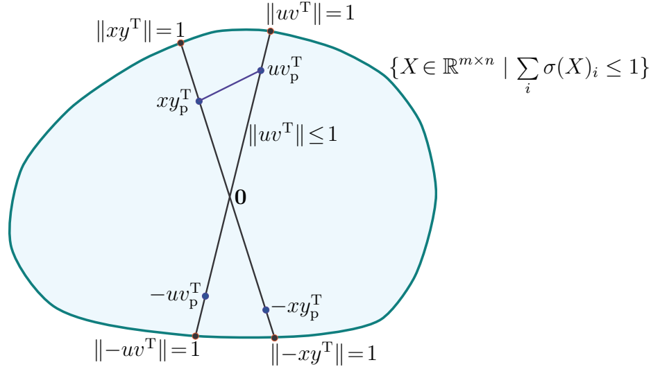
Figure 23: uv_p^T is a convex combination of normalized dyads \|\pm uv^T\| = 1 ; similarly for xy_p^T . Any point in line segment joining xy_p^T to uv_p^T is expressible as a convex combination of two to four points indicated on boundary.
