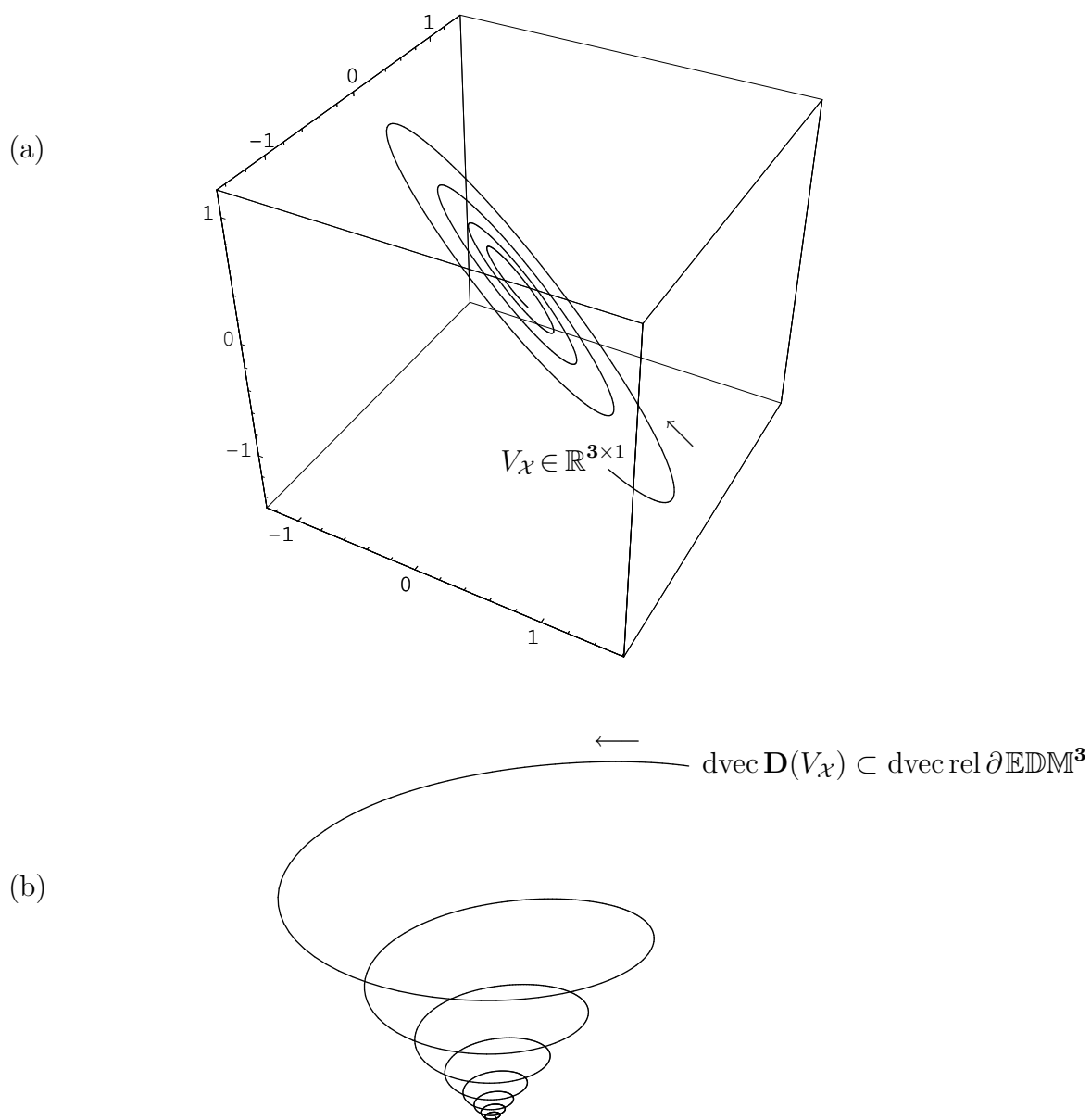
Figure 146: (a) Vector V_{\mathcal{X}} from Figure 145 spirals in \mathcal{N}(\mathbf{1}^T) \subset \mathbb{R}^3 decaying toward origin. (Spiral is two-dimensional in vector space \mathbb{R}^3 .) (b) Corresponding trajectory \mathbf{D}(V_{\mathcal{X}}) on EDM cone relative boundary creates a vortex also decaying toward origin. There are two complete orbits on EDM cone boundary about axis of revolution for every single revolution of V_{\mathcal{X}} about origin. (Vortex is three-dimensional in isometrically isomorphic \mathbb{R}^3 .)
