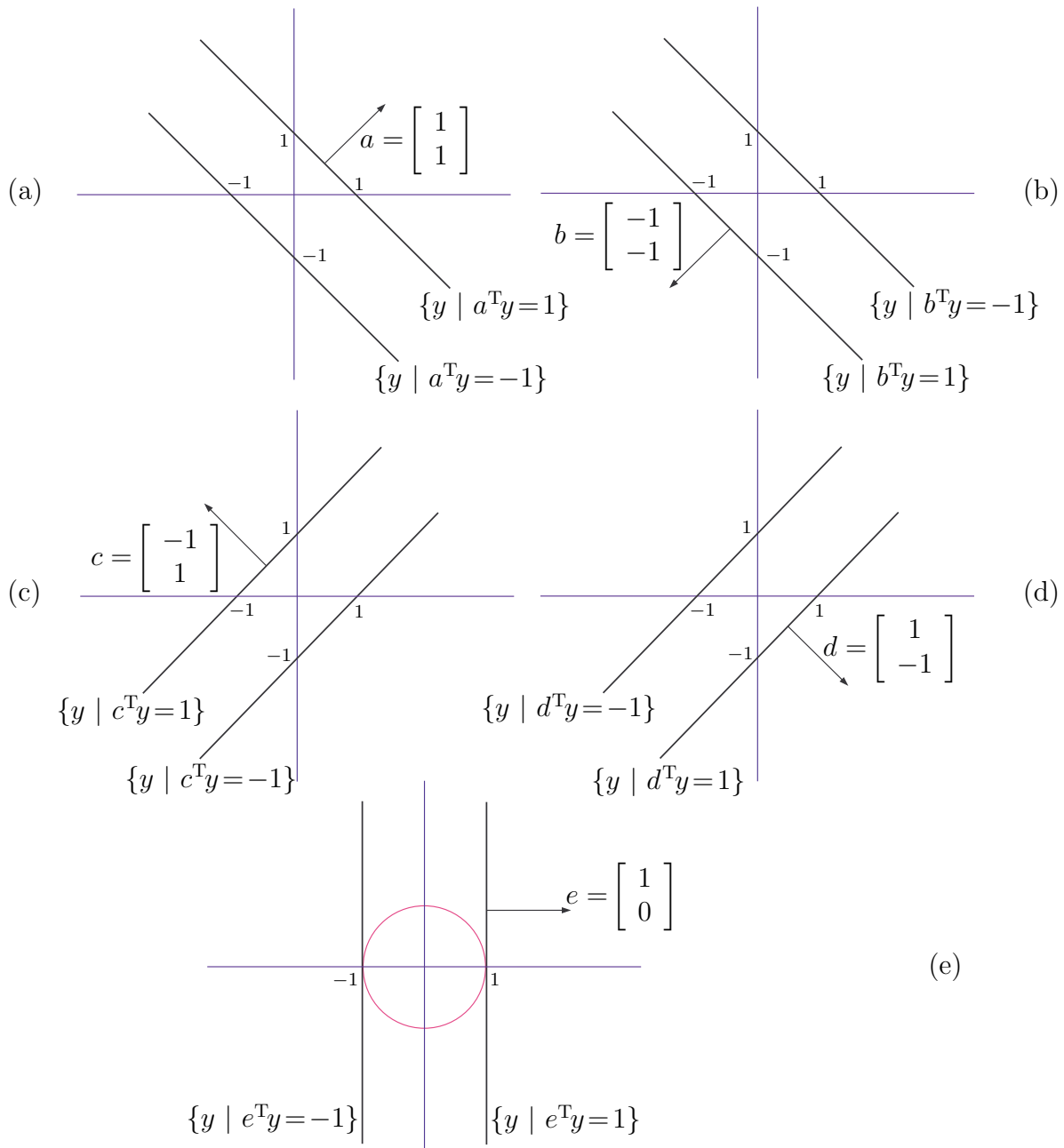
Figure 26: (a)-(d) Hyperplanes in \mathbb{R}^2 (truncated) redundantly emphasize: hyperplane movement opposite to its normal direction minimizes vector inner-product. This concept is exploited to attain analytical solution of linear programs by visual inspection; e.g. , Example 2.4.2.6.2, Exercise 2.5.1.2.2, Example 3.4.0.0.2, [61, exer.4.8-exer.4.20]. Each graph is also interpretable as contour plot of a real affine function of two variables as in Figure 73. (e) |\beta|/\|\alpha\| from \partial\mathcal{H} = \{x \mid \alpha^T x = \beta\} represents radius of hypersphere about \mathbf{0} supported by any hyperplane with same ratio |inner product|/norm.
