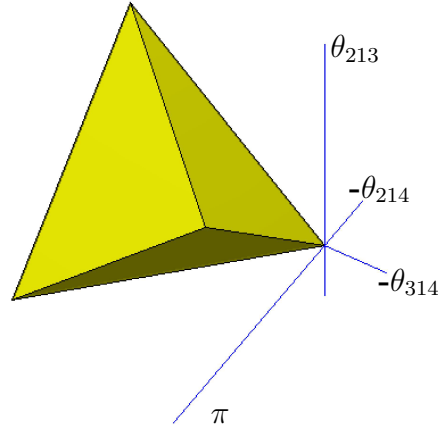
Figure 142: The relative-angle inequality tetrahedron (1196) bounding \text{EDM}^4 is regular; drawn in entirety. Each angle \theta (987) must belong to this solid to be realizable.
