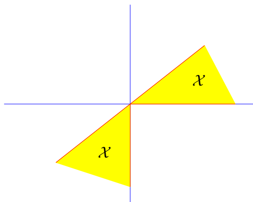
Figure 37: Truncated nonconvex cone \mathcal{X} = \{x \in \mathbb{R}^2 \mid x_1 \geq x_2, x_1 x_2 \geq 0\} . Boundary is also a cone. [251, §2.4] Cartesian axes drawn for reference. Each half (about the origin) is itself a convex cone.
