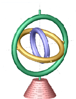
Figure 165: Gimbal : a mechanism imparting three degrees of dimensional freedom to a Euclidean body suspended at the device's center. Each ring is free to rotate about one axis. (Courtesy of The MathWorks Inc.)
