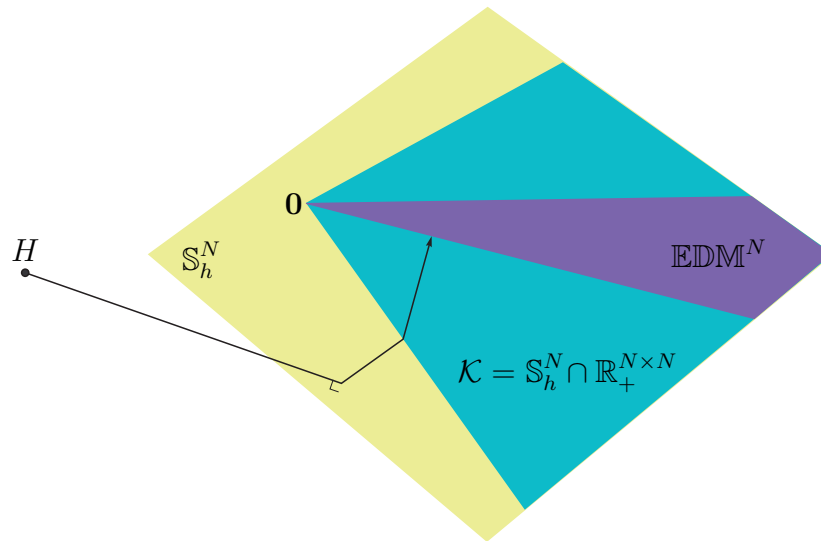
Figure 159: Pseudo-Venn diagram from Figure 158 showing elbow placed in path of projection of H on \text{EDM}^N \subset S_h^N by an optimization problem demanding nonnegative input matrix H . The first two line segments leading away from H result from correct order-of-projection required to provide nonnegative H prior to optimization. Were H nonnegative, then its projection on S_h^N would instead belong to \mathcal{K} ; making the elbow disappear. (confer Figure 173)
