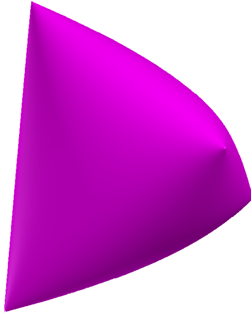
Figure 136: Elliptope \mathcal{E}^3 in isometrically isomorphic \mathbb{R}^6 (projected on \mathbb{R}^3 ) is a convex body that appears to possess some kind of symmetry in this dimension; it resembles a malformed pillow in the shape of a bulging tetrahedron. Elliptope relative boundary is not smooth and comprises all set members (1109) having at least one 0 eigenvalue. [239, §2.1] This elliptope has an infinity of vertices, but there are only four vertices corresponding to a rank-1 matrix. Those yy^T , evident in the illustration, have binary vector y \in \mathbb{R}^3 with entries in \{\pm 1\} .
