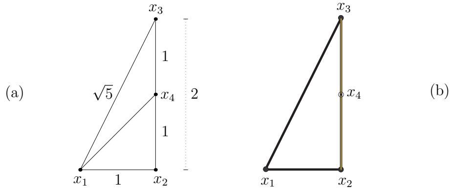
Figure 122: (a) Complete dimensionless EDM graph . (b) Emphasizing obscured segments \overline{x_2x_4} , \overline{x_4x_3} , and \overline{x_2x_3} , now only five (2N - 3) absolute distances are specified. EDM so represented is incomplete, missing d_{14} as in (915), yet the isometric reconstruction (§5.4.2.3.7) is unique as proved in §5.9.3.0.1 and §5.14.4.1.1. First four properties of Euclidean metric are not a recipe for reconstruction of this polyhedron.
