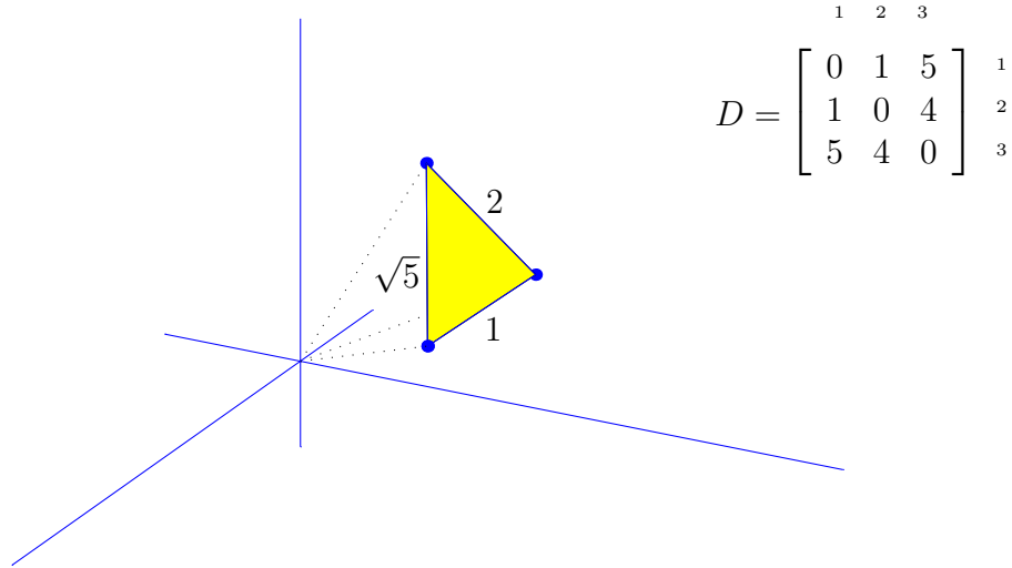
Figure 121: Convex hull of three points ( N=3 ) is shaded in \mathbb{R}^3 ( n=3 ). Dotted lines are imagined vectors to points whose affine dimension is 2.
