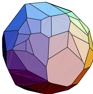
Figure 20: Convex hull of a random list of points in \mathbb{R}^3 . Some points from that generating list reside interior to this convex polyhedron (§2.12). [375, Convex Polyhedron ] (Avis-Fukuda-Mizukoshi)
