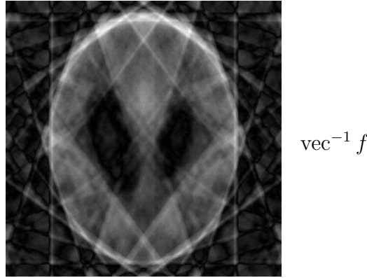
Figure 109: Aliasing of Shepp-Logan phantom in Figure 107 resulting from \mathbb{k} -space subsampling pattern in Figure 108. This image is real because binary mask \Phi is vertically and horizontally symmetric. It is remarkable that the phantom can be reconstructed, by convex iteration, given only \mathcal{U}_0 = \text{vec}^{-1} f .
