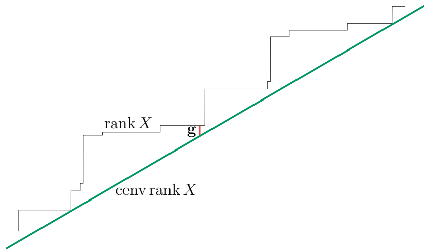
Figure 160: Abstraction of convex envelope of rank function. Rank is a quasiconcave function on positive semidefinite cone, but its convex envelope is the largest convex function whose epigraph contains it. Vertical bar labelled \mathbf{g} measures a trace/rank gap; id est , rank found always exceeds estimate; large decline in trace required here for only small decrease in rank.
