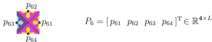
Figure 114: Demo-game piece P_6 illustrating edge-color \bullet p_{6j} \in \mathbb{R}^L counterclockwise ordering in j beginning from right.
