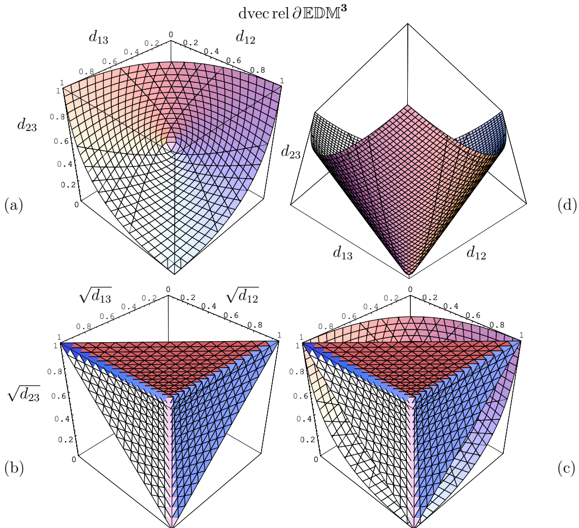
Figure 144: Relative boundary (tiled) of EDM cone \mathbb{EDM}^3 drawn truncated in isometrically isomorphic subspace \mathbb{R}^3 . (a) EDM cone drawn in usual distance-square coordinates d_{ij} . View is from interior toward origin. Unlike positive semidefinite cone, EDM cone is not selfdual; neither is it proper in ambient symmetric subspace (dual EDM cone for this example belongs to isomorphic \mathbb{R}^6 ). (b) Drawn in its natural coordinates \sqrt{d_{ij}} (absolute distance), cone remains convex ( confer §5.10); intersection of three halfspaces (1095) whose partial boundaries each contain origin. Cone geometry becomes nonconvex (nonpolyhedral) in higher dimension. (§6.3) (c) Two coordinate systems artificially superimposed. Coordinate transformation from d_{ij} to \sqrt{d_{ij}} appears a topological contraction. (d) Sitting on its vertex \mathbf{0} , pointed \mathbb{EDM}^3 is a circular cone having axis of revolution \text{dvec}(-E) = \text{dvec}(\mathbf{1}\mathbf{1}^T - I) (1128) (73). (Rounded vertex is plot artifact.)
