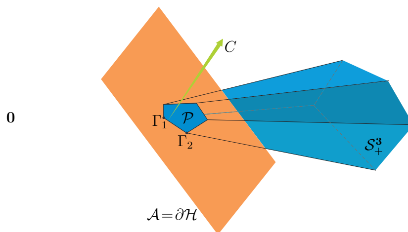
Figure 65: Visualizing positive semidefinite cone in high dimension: Proper polyhedral cone \mathcal{S}_+^3 \subset \mathbb{R}^3 representing positive semidefinite cone \mathbb{S}_+^3 \subset \mathbb{S}^3 ; analogizing its intersection with hyperplane \mathbb{S}_+^3 \cap \partial\mathcal{H} . Number of facets is arbitrary (analogy is not inspired by eigen decomposition). The rank-0 positive semidefinite matrix corresponds to the origin in \mathbb{R}^3 , rank-1 positive semidefinite matrices correspond to the edges of the polyhedral cone, rank-2 to the facet relative interiors, and rank-3 to the polyhedral cone interior. Vertices \Gamma_1 and \Gamma_2 are extreme points of polyhedron \mathcal{P} = \partial\mathcal{H} \cap \mathcal{S}_+^3 , and extreme directions of \mathcal{S}_+^3 . A given vector C is normal to another hyperplane (not illustrated but independent w.r.t \partial\mathcal{H} ) containing line segment \overline{\Gamma_1\Gamma_2} minimizing real linear function \langle C, X \rangle on \mathcal{P} . (confer Figure 19)
