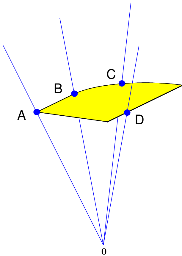
Figure 32: Properties of extreme points carry over to extreme directions. [255, §18] Four rays (drawn truncated) on boundary of conic hull of two-dimensional closed convex set from Figure 23 lifted to \mathbb{R}^3 . Ray through point A is exposed hence extreme. Extreme direction B on cone boundary is not an exposed direction, although it belongs to the exposed face \text{cone}\{A, B\} . Extreme ray through C is exposed. Point D is neither an exposed or extreme direction although it belongs to a two-dimensional exposed face of the conic hull.
