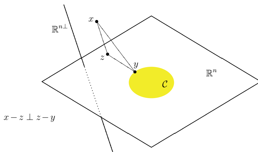
Figure 133: Closed convex set \mathcal{C} belongs to subspace \mathbb{R}^n (shown bounded in sketch and drawn without proper perspective). Point y is unique minimum-distance projection of x on \mathcal{C} ; equivalent to product of orthogonal projection of x on \mathbb{R}^n and minimum-distance projection of result z on \mathcal{C} .
