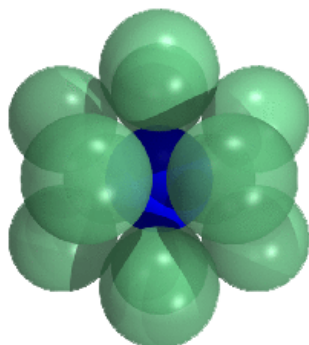
Figure 88: Sphere-packing illustration from [315, kissing number ]. Translucent balls illustrated all have the same diameter.
