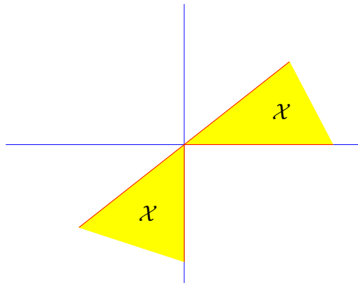
Figure 28: Truncated nonconvex cone \mathcal{X} = \{x \in \mathbb{R}^2 \mid x_1 \geq x_2, x_1 x_2 \geq 0\} . Boundary is also a cone. [205, §2.4] Cartesian axes drawn for reference. Each half (about the origin) is itself a convex cone.
