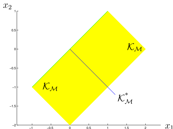
Figure 53: Monotone cone \mathcal{K}_{\mathcal{M}} and its dual \mathcal{K}_{\mathcal{M}}^* (drawn truncated) in \mathbb{R}^2 .
