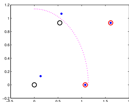
Figure 71: Typical solution for 2-lattice in Figure 66 with noise factor \eta = 0.1 . Two red rightmost nodes are anchors; two remaining nodes are sensors. Radio range of sensor 1 indicated by arc; radius = 1.14. Actual sensor indicated by target \circ while its localization is indicated by bullet \bullet . Rank-2 solution found in 1 iteration (668) (1571a) subject to reflection error.
