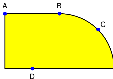
Figure 23: Closed convex set in \mathbb{R}^2 . Point A is exposed hence extreme; a classical vertex. Point B is extreme but not an exposed point. Point C is exposed and extreme; zero-dimensional exposure makes it a vertex. Point D is neither an exposed or extreme point although it belongs to a one-dimensional exposed face. [165, §A.2.4] [275, §3.6] Closed face \overline{AB} is exposed; a facet. The arc is not a conventional face, yet it is composed entirely of extreme points. Union of all rotations of this entire set about its vertical edge produces another convex set in three dimensions having no edges; but that convex set produced by rotation about horizontal edge containing D has edges.
