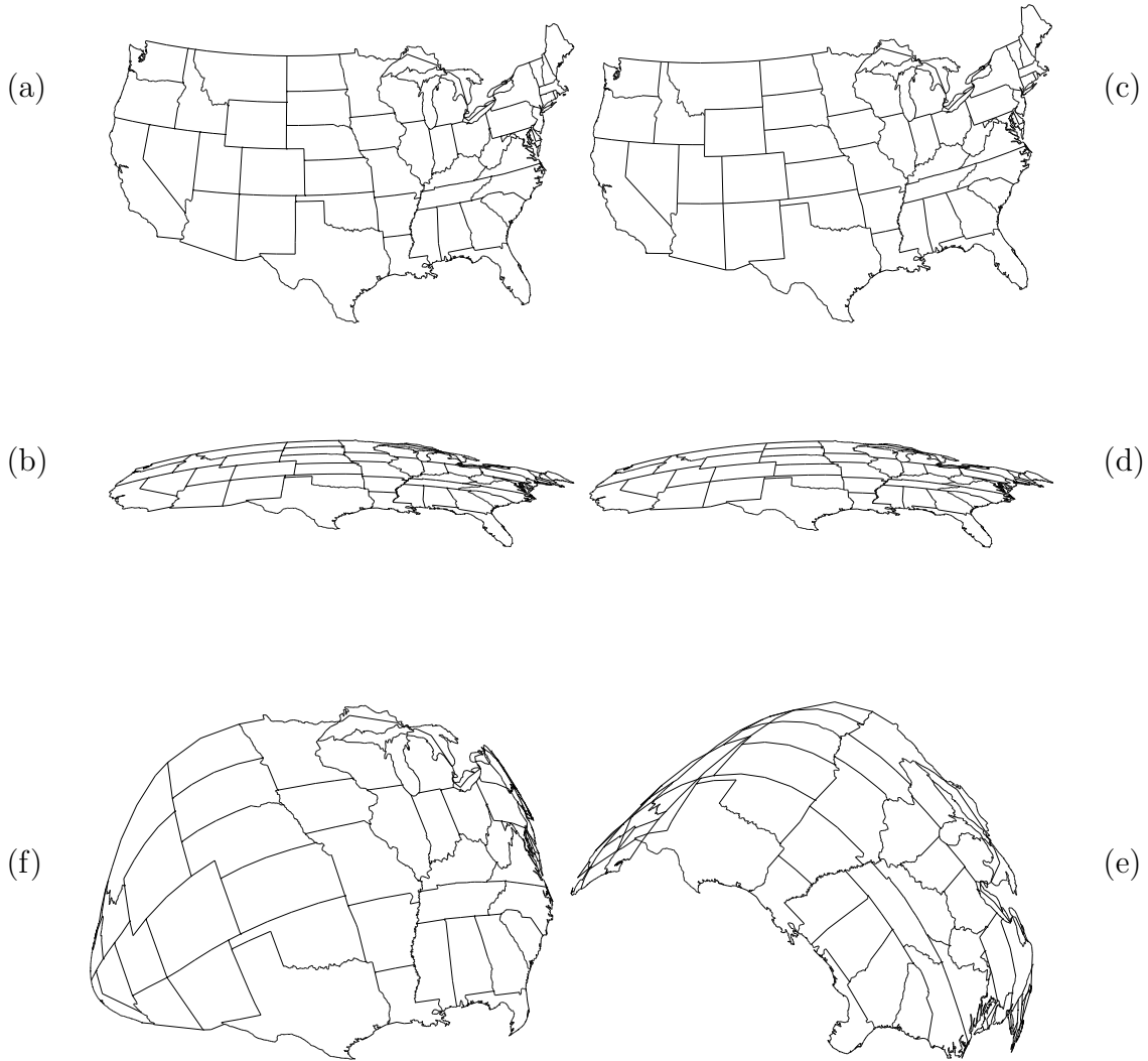
Figure 102: Map of United States of America showing some state boundaries and the Great Lakes. All plots made by connecting 5020 points. Any difference in scale in (a) through (d) is artifact of plotting routine.
