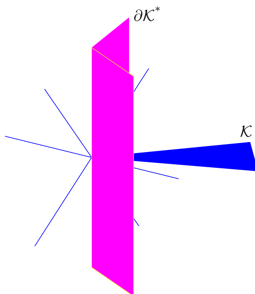
Figure 31: \mathcal{K} is a pointed polyhedral cone having empty interior in \mathbb{R}^3 (drawn truncated and in a plane parallel to the floor upon which you stand). \mathcal{K}^* is a wedge whose truncated boundary is illustrated (drawn perpendicular to the floor). In this particular instance, \mathcal{K} \subset \text{int } \mathcal{K}^* (excepting the origin). Cartesian coordinate axes drawn for reference.
