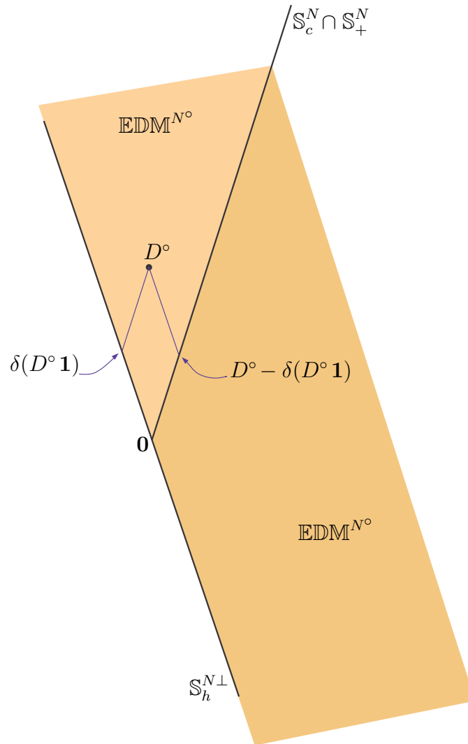
Figure 118: Hand-drawn abstraction of polar EDM cone (drawn truncated). Any member D^\circ of polar EDM cone can be decomposed into two linearly independent nonorthogonal components: \delta(D^\circ \mathbf{1}) and D^\circ - \delta(D^\circ \mathbf{1}) .
