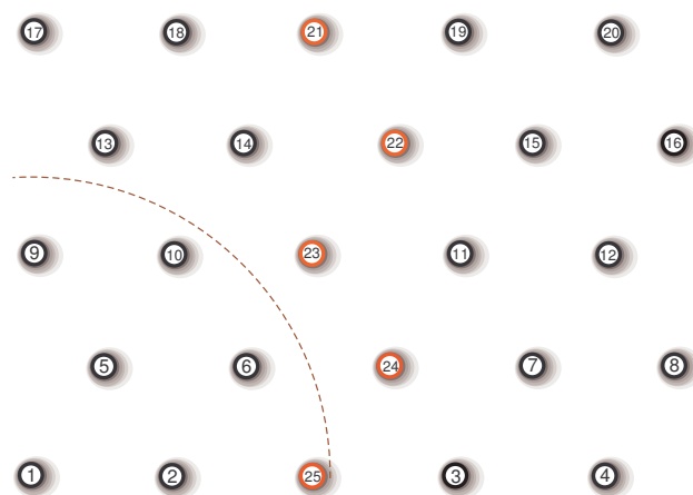
Figure 69: 5-lattice in \mathbb{R}^2 . Nodes 21 through 25 are anchors.
