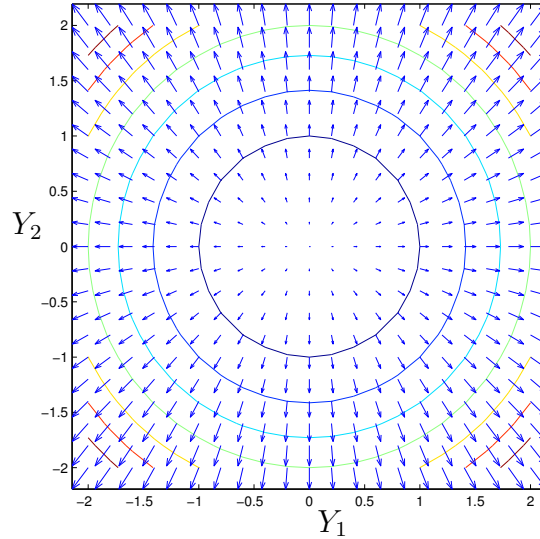
Figure 61: Gradient in \mathbb{R}^2 evaluated on grid over some open disc in domain of convex quadratic bowl f(Y) = Y^T Y : \mathbb{R}^2 \rightarrow \mathbb{R} illustrated in Figure 62. Circular contours are level sets; each defined by a constant function-value.
