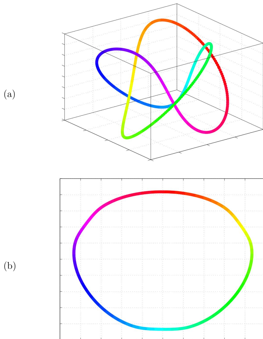
Figure 109: (a) Trefoil knot in \mathbb{R}^3 from Weinberger & Saul [314]. (b) Topological transformation algorithm employing 4 nearest neighbors and N = 539 samples reduces affine dimension of knot to r = 2 . Choosing instead 2 nearest neighbors would make this embedding more circular.
