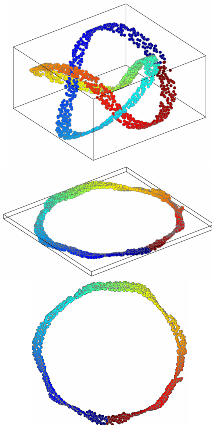
Figure 110: Trefoil ribbon ; courtesy, Kilian Weinberger. Same topological transformation algorithm with 5 nearest neighbors and N = 1617 samples.
