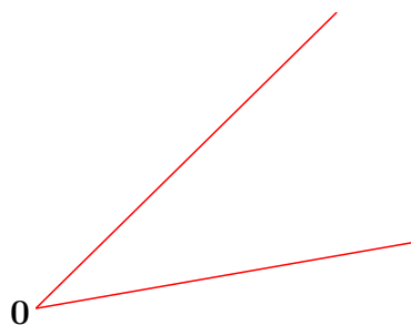
Figure 26: Boundary of a convex cone in \mathbb{R}^2 is a nonconvex cone; a pair of rays emanating from the origin.
