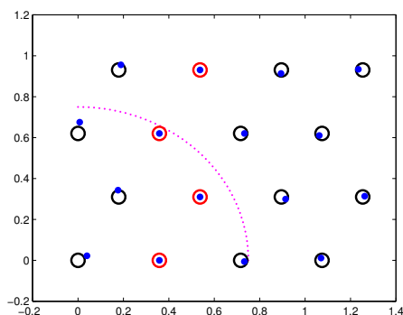
Figure 73: Typical solution for 4-lattice in Figure 68 with noise factor \eta = 0.1 . Four red vertical middle-left nodes are anchors; remaining nodes are sensors. Radio range of sensor 1 indicated by arc; radius = 0.75. Actual sensor indicated by target \circ while its localization is indicated by bullet \bullet . Rank-2 solution found in 7 iterations (668) (1571a).
