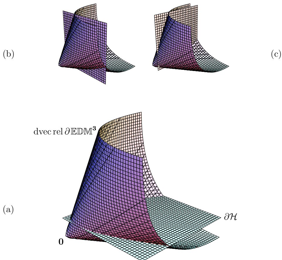
Figure 107: (a) In isometrically isomorphic subspace \mathbb{R}^3 , intersection of \text{EDM}^3 with hyperplane \partial\mathcal{H} representing one fixed symmetric entry d_{23} = \kappa (both drawn truncated, rounded vertex is artifact of plot). EDMs in this dimension corresponding to affine dimension 1 comprise relative boundary of EDM cone (§6.6). Since intersection illustrated includes a nontrivial subset of cone's relative boundary, then it is apparent there exist infinitely many EDM completions corresponding to affine dimension 1. In this dimension it is impossible to represent a unique nonzero completion corresponding to affine dimension 1, for example, using a single hyperplane because any hyperplane supporting relative boundary at a particular point \Gamma contains an entire ray \{\zeta\Gamma \mid \zeta \geq 0\} belonging to \text{rel } \partial\text{EDM}^3 by Lemma 2.8.0.0.1. (b) d_{13} = \kappa . (c) d_{12} = \kappa .
