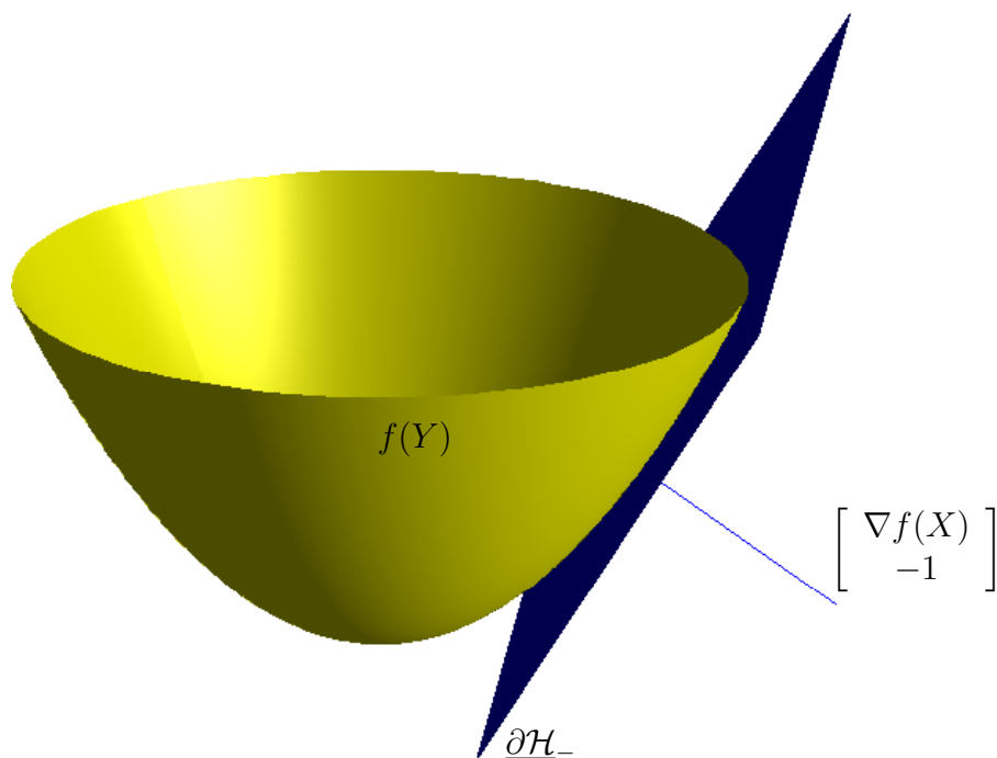
Figure 62: When a real function f is differentiable at each point in its open domain, there is an intuitive geometric interpretation of function convexity in terms of its gradient \nabla f and its epigraph: Drawn is a convex quadratic bowl in \mathbb{R}^2 \times \mathbb{R} (confer Figure 128, p.602); f(Y) = Y^T Y : \mathbb{R}^2 \rightarrow \mathbb{R} versus Y on some open disc in \mathbb{R}^2 . Unique strictly supporting hyperplane \partial\mathcal{H}_- \in \mathbb{R}^2 \times \mathbb{R} (only partially drawn) and its normal vector [\nabla f(X)^T \ -1]^T at the particular point of support [X^T \ f(X)]^T are illustrated. The interpretation: At each and every coordinate Y , there is such a hyperplane containing [Y^T \ f(Y)]^T and supporting the epigraph.
