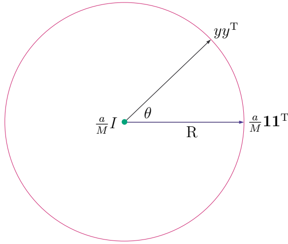
Figure 37: Illustrated is a section, perpendicular to axis of revolution, of circular cone from Figure 36. Radius R is distance from any extreme direction to axis at \frac{a}{M}I . Vector \frac{a}{M}\mathbf{1}\mathbf{1}^T is an arbitrary reference by which to measure angle \theta .
