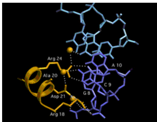
Figure 95: A depiction of molecular conformation. [94]
