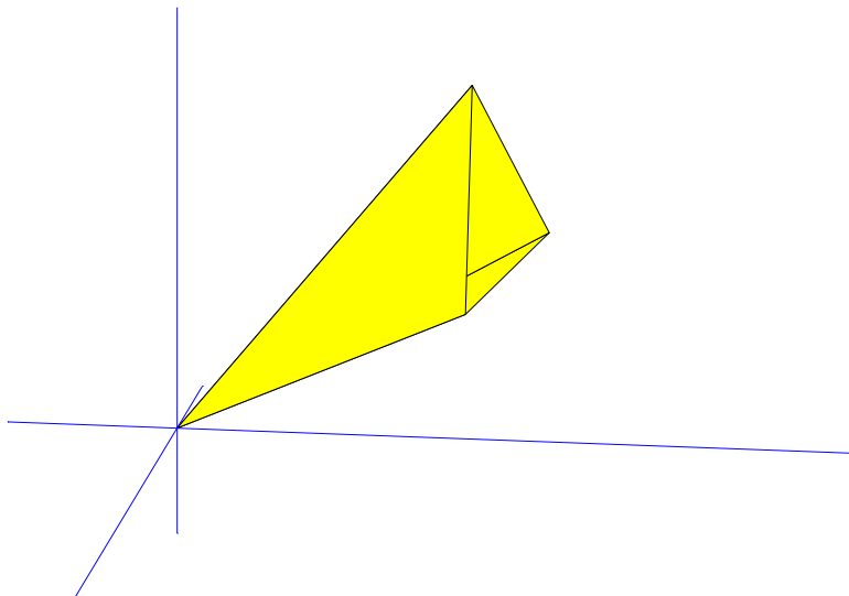
Figure 17: A simplicial cone (§2.12.3.1.1) in \mathbb{R}^3 whose boundary is drawn truncated; constructed using A \in \mathbb{R}^{3 \times 3} and C = \mathbf{0} in (255). By the most fundamental definition of a cone (§2.7.1), entire boundary can be constructed from an aggregate of rays emanating exclusively from the origin. Each of three extreme directions corresponds to an edge (§2.6.0.0.3); they are conically, affinely, and linearly independent for this cone. Because this set is polyhedral, exposed directions are in one-to-one correspondence with extreme directions; there are only three. Its extreme directions give rise to what is called a vertex-description of this polyhedral cone; simply, the conic hull of extreme directions. Obviously this cone can also be constructed by intersection of three halfspaces; hence the equivalent halfspace-description .
