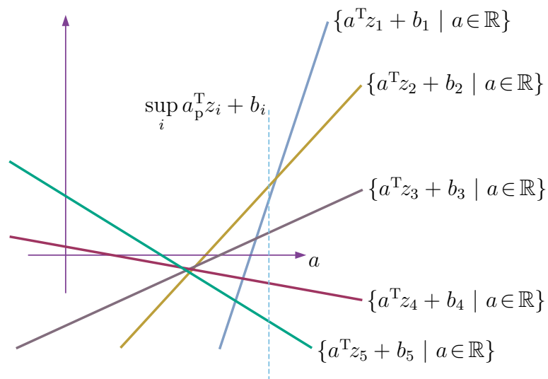
Figure 59: Pointwise supremum of convex functions remains a convex function. Illustrated is a supremum of affine functions in variable a evaluated for a particular argument a_p . Topmost affine function is supremum for each value of a .
