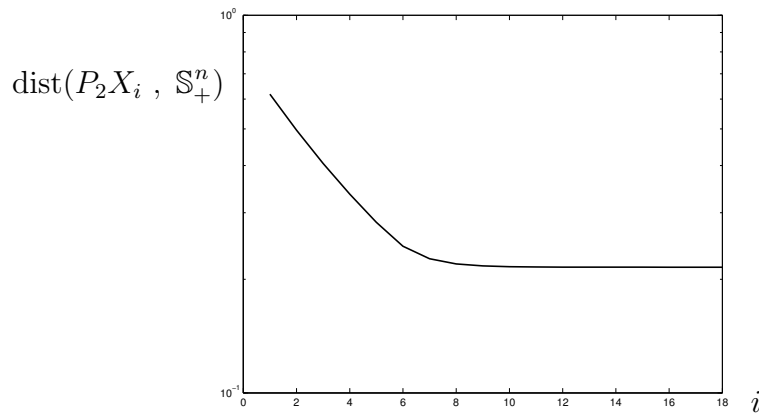
Figure 139: Distance ( confer (1943)) between PSD cone and iterate (1946) in affine subset \mathcal{A} (1939) for Laurent’s completion problem; initially, decreasing geometrically.
