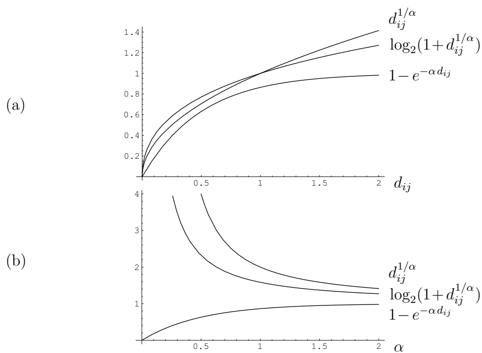
Figure 101: Some entrywise EDM compositions: (a) \alpha = 2 . Concave nondecreasing in d_{ij} . (b) Trajectory convergence in \alpha for d_{ij} = 2 .
