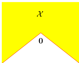
Figure 27: Nonconvex cone \mathcal{X} drawn truncated in \mathbb{R}^2 . Boundary is also a cone. [205, §2.4] Cone exterior is convex cone.
