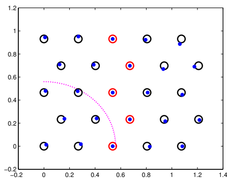
Figure 74: Typical solution for 5-lattice in Figure 69 with noise factor \eta = 0.1 . Five red vertical middle nodes are anchors; remaining nodes are sensors. Radio range of sensor 1 indicated by arc; radius = 0.56. Actual sensor indicated by target \circ while its localization is indicated by bullet \bullet . Rank-2 solution found in 3 iterations (668) (1571a).
