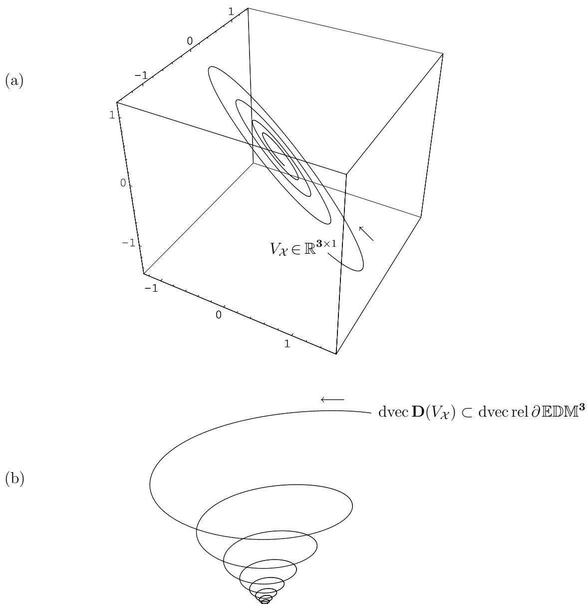
Figure 112: (a) Vector V_{\mathcal{X}} from Figure 111 spirals in \mathcal{N}(\mathbf{1}^T) \subset \mathbb{R}^3 decaying toward origin. (Spiral is two-dimensional in vector space \mathbb{R}^3 .) (b) Corresponding trajectory \mathbf{D}(V_{\mathcal{X}}) on EDM cone relative boundary creates a vortex also decaying toward origin. There are two complete orbits on EDM cone boundary about axis of revolution for every single revolution of V_{\mathcal{X}} about origin. (Vortex is three-dimensional in isometrically isomorphic \mathbb{R}^3 .)
