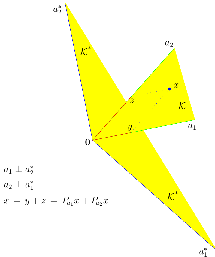
Figure 131: ( confer Figure 51) Biorthogonal expansion of point x \in \text{aff } \mathcal{K} is found by projecting x nonorthogonally on extreme directions of polyhedral cone \mathcal{K} \subset \mathbb{R}^2 . (Dotted lines of projection bound this translated negated cone.) Direction of projection on extreme direction a_1 is orthogonal to extreme direction a_1^* of dual cone \mathcal{K}^* and parallel to a_2 (§E.3.5); similarly, direction of projection on a_2 is orthogonal to a_2^* and parallel to a_1 . Point x is sum of nonorthogonal projections: x on \mathcal{R}(a_1) and x on \mathcal{R}(a_2) . Expansion is unique because extreme directions of \mathcal{K} are linearly independent. Were a_1 orthogonal to a_2 , then \mathcal{K} would be identical to \mathcal{K}^* and nonorthogonal projections would become orthogonal.
