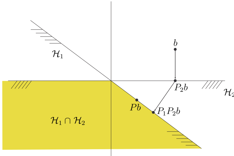
Figure 135: The sets \{\mathcal{C}_k\} in this example comprise two halfspaces \mathcal{H}_1 and \mathcal{H}_2 . The von Neumann-style alternating projection in \mathbb{R}^2 quickly converges to P_1 P_2 b (feasibility). The unique minimum-distance projection on the intersection is, of course, Pb .
