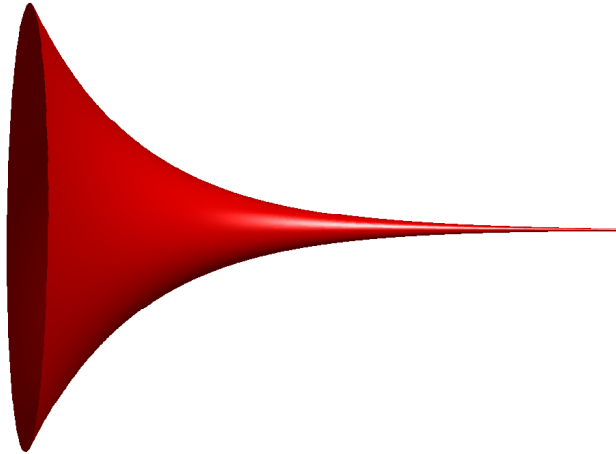
Figure 29: Not a cone; ironically, the three-dimensional flared horn (with or without its interior) resembling the mathematical symbol \succ denoting cone membership and partial order.
