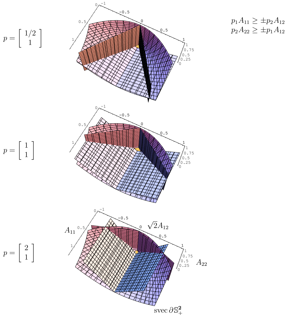
Figure 38: Proper polyhedral cone \mathcal{K} , created by intersection of halfspaces, inscribes PSD cone in isometrically isomorphic \mathbb{R}^3 as predicted by Geršgorin discs theorem for A=[A_{ij}] \in \mathbb{S}^2 . Hyperplanes supporting \mathcal{K} intersect along boundary of PSD cone. Four extreme directions of \mathcal{K} coincide with extreme directions of PSD cone.
