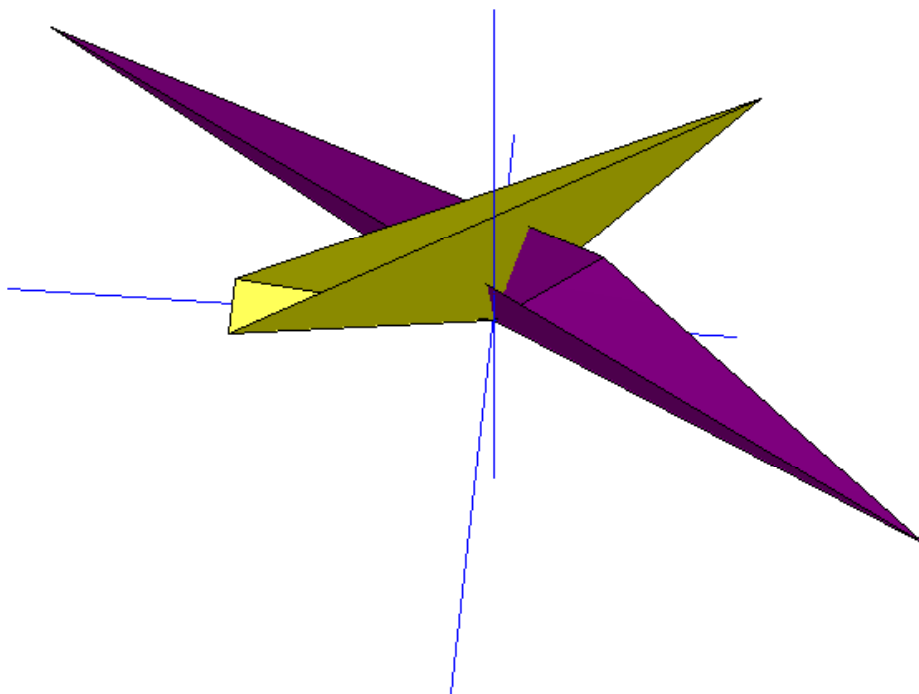
Figure 43: Two views of a simplicial cone and its dual in \mathbb{R}^3 (second view on next page). Semi-infinite boundary of each cone is truncated for illustration. Each cone has three facets ( confer §2.13.11.0.3). Cartesian axes are drawn for reference.
