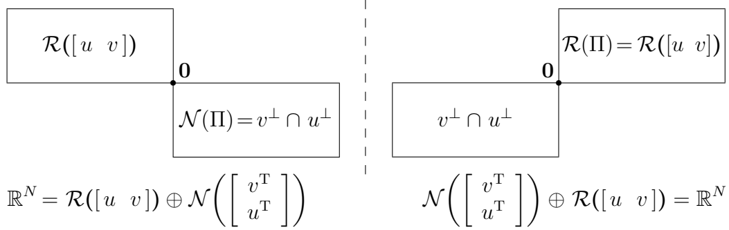
Figure 125: Four fundamental subspaces [279, §3.6] of a doublet \Pi = uv^T + vu^T \in \mathbb{S}^N . \Pi(x) = (uv^T + vu^T)x is a linear bijective mapping from \mathcal{R}([u \ v]) to \mathcal{R}([u \ v]) .
