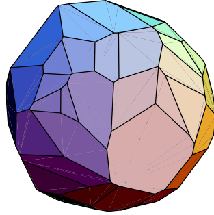
Figure 14: Convex hull of a random list of points in \mathbb{R}^3 . Some points from that generating list reside interior to this convex polyhedron . [315, Convex Polyhedron ] (Avis-Fukuda-Mizukoshi)
