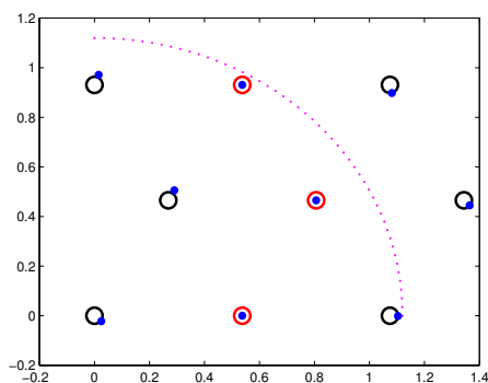
Figure 72: Typical solution for 3-lattice in Figure 67 with noise factor \eta = 0.1 . Three red vertical middle nodes are anchors; remaining nodes are sensors. Radio range of sensor 1 indicated by arc; radius = 1.12. Actual sensor indicated by target \circ while its localization is indicated by bullet \bullet . Rank-2 solution found in 2 iterations (668) (1571a).
