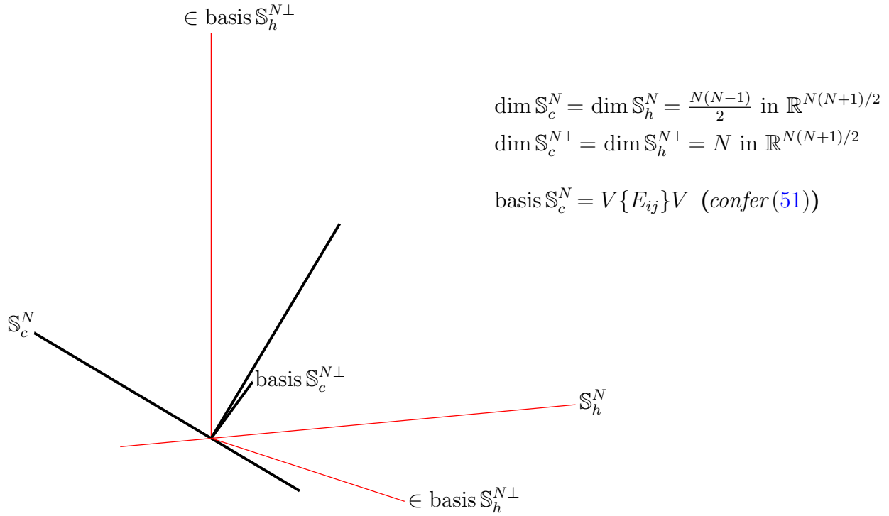
Figure 97: Orthogonal complements in \mathbb{S}^N abstractly oriented in isometrically isomorphic \mathbb{R}^{N(N+1)/2} . Case N=2 accurately illustrated in \mathbb{R}^3 . Orthogonal projection of basis for \mathbb{S}_h^{N\perp} on \mathbb{S}_c^{N\perp} yields another basis for \mathbb{S}_c^{N\perp} . (Basis vectors for \mathbb{S}_c^{N\perp} are illustrated lying in a plane orthogonal to \mathbb{S}_c^N in this dimension. Basis vectors for each \perp space outnumber those for its respective orthogonal complement; such is not the case in higher dimension.)
