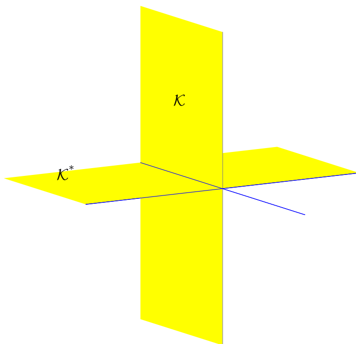
Figure 49: \mathcal{K} and \mathcal{K}^* are halfplanes in \mathbb{R}^3 ; blades . Both semi-infinite convex cones appear truncated. Each cone is like \mathcal{K} in Figure 46, but embedded in a two-dimensional subspace of \mathbb{R}^3 . Cartesian coordinate axes drawn for reference.
