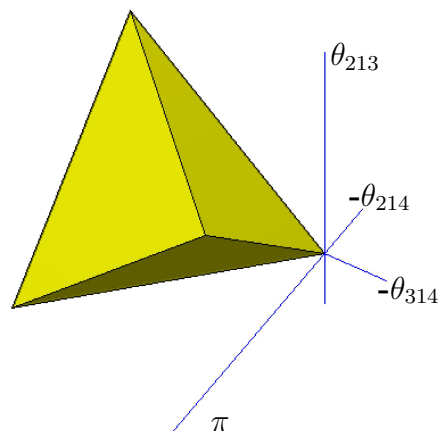
Figure 104: The relative-angle inequality tetrahedron (1056) bounding \mathbb{EDM}^4 is regular; drawn in entirety. Each angle \theta (848) must belong to this solid to be realizable.
