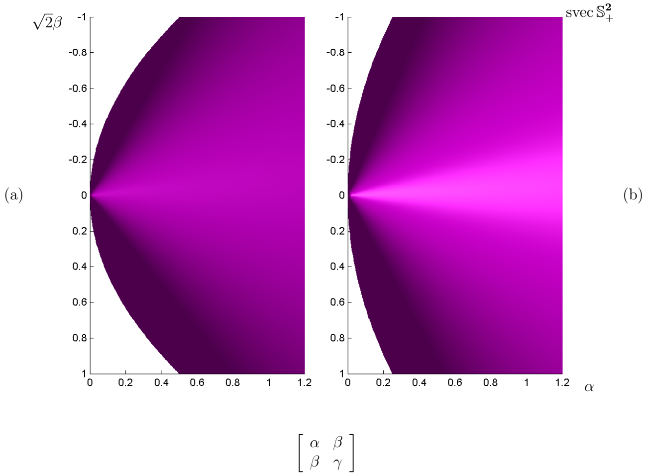
Figure 35: (a) Projection of the PSD cone \mathbb{S}_+^2 , truncated above \gamma=1 , on \alpha\beta -plane in isometrically isomorphic \mathbb{R}^3 . View is from above with respect to Figure 33. (b) Truncated above \gamma=2 . From these plots we may infer, for example, the line \{[0 \ 1/\sqrt{2} \ \gamma]^T \mid \gamma \in \mathbb{R}\} intercepts the PSD cone at some large value of \gamma ; in fact, \gamma=\infty .
