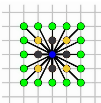
Figure 81: Neighboring-pixel candidates from [298] for estimating image-gradient. Our implementation selects adaptively from darkest four • about central.
