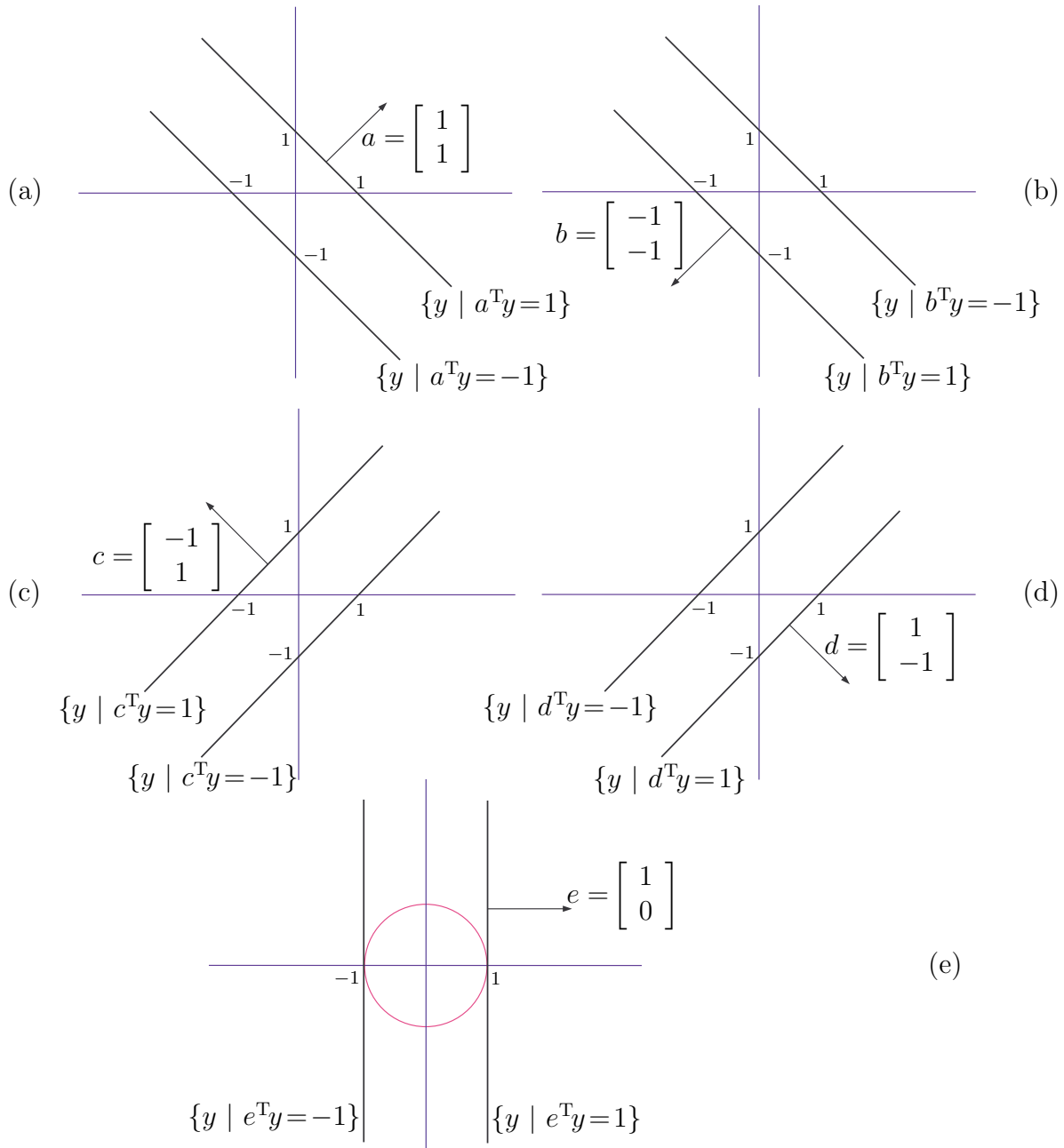
Figure 19: (a)-(d) Hyperplanes in \mathbb{R}^2 (truncated). Movement in normal direction increases vector inner-product. This visual concept is exploited to attain analytical solution of linear programs; e.g. , Example 2.4.2.6.2, Example 3.1.6.0.1, [51, exer.4.8-exer.4.20]. Each graph is also interpretable as a contour plot of a real affine function of two variables as in Figure 58. (e) Ratio |b|/\|a\| from \{x \mid a^T x = b\} represents radius of hypersphere about \mathbf{0} supported by hyperplane whose normal is a .
