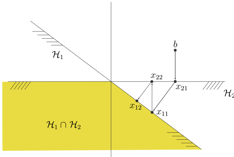
Figure 140: \mathcal{H}_1 and \mathcal{H}_2 are the same halfspaces as in Figure 135. Dykstra's alternating projection algorithm generates the alternations b, x_{21}, x_{11}, x_{22}, x_{12}, x_{12} \dots x_{12} . The path illustrated from b to x_{12} in \mathbb{R}^2 terminates at the desired result, Pb in Figure 135. The \{y_{ki}\} correspond to the first two difference vectors drawn (in the first iteration i=1 ), then oscillate between zero and a negative vector thereafter. These alternations are not so robust in presence of noise as for the example in Figure 134.
