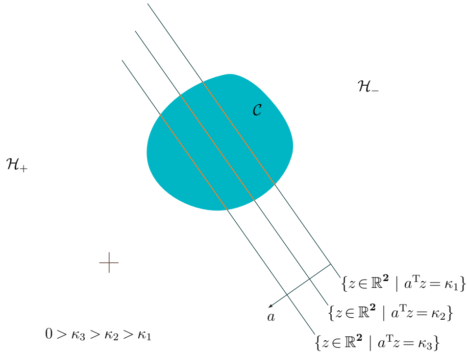
Figure 21: Each shaded line segment \{z \in \mathcal{C} \mid a^T z = \kappa_i\} belonging to set \mathcal{C} \subset \mathbb{R}^2 shows intersection with hyperplane parametrized by scalar \kappa_i ; each shows a (linear) contour in vector z of equal inner product with normal vector a . Cartesian axes drawn for reference. (confer Figure 58)
