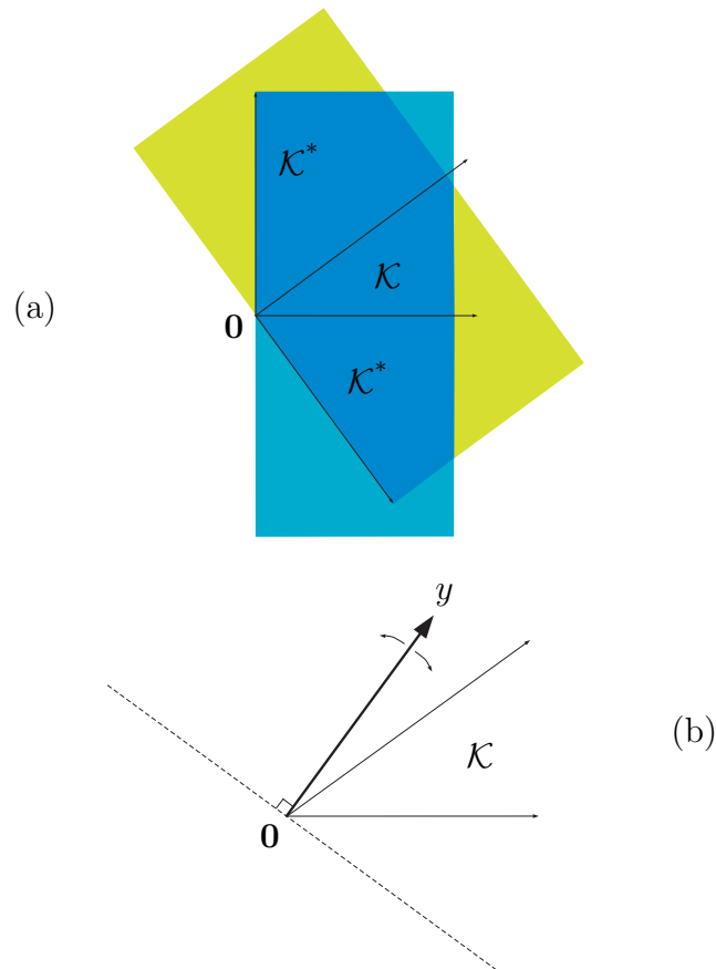
Figure 44: Two equivalent constructions of dual cone \mathcal{K}^* in \mathbb{R}^2 : (a) Showing construction by intersection of halfspaces about \mathbf{0} (drawn truncated). Only those two halfspaces whose bounding hyperplanes have inward-normal corresponding to an extreme direction of this pointed closed convex cone \mathcal{K} \subset \mathbb{R}^2 need be drawn; by (329). (b) Suggesting construction by union of inward-normals y to each and every hyperplane \partial\mathcal{H}_+ supporting \mathcal{K} . This interpretation is valid when \mathcal{K} is convex because existence of a supporting hyperplane is then guaranteed (§2.4.2.6).
