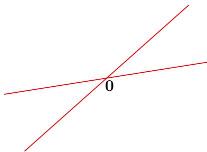
Figure 25: This nonconvex cone in \mathbb{R}^2 is a pair of lines through the origin. [205, §2.4]
