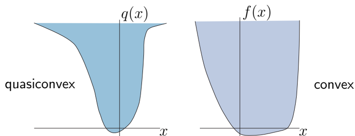
Figure 60: Quasiconvex function q epigraph is not necessarily convex, but convex function f epigraph is convex in any dimension. Sublevel sets are necessarily convex for either.
