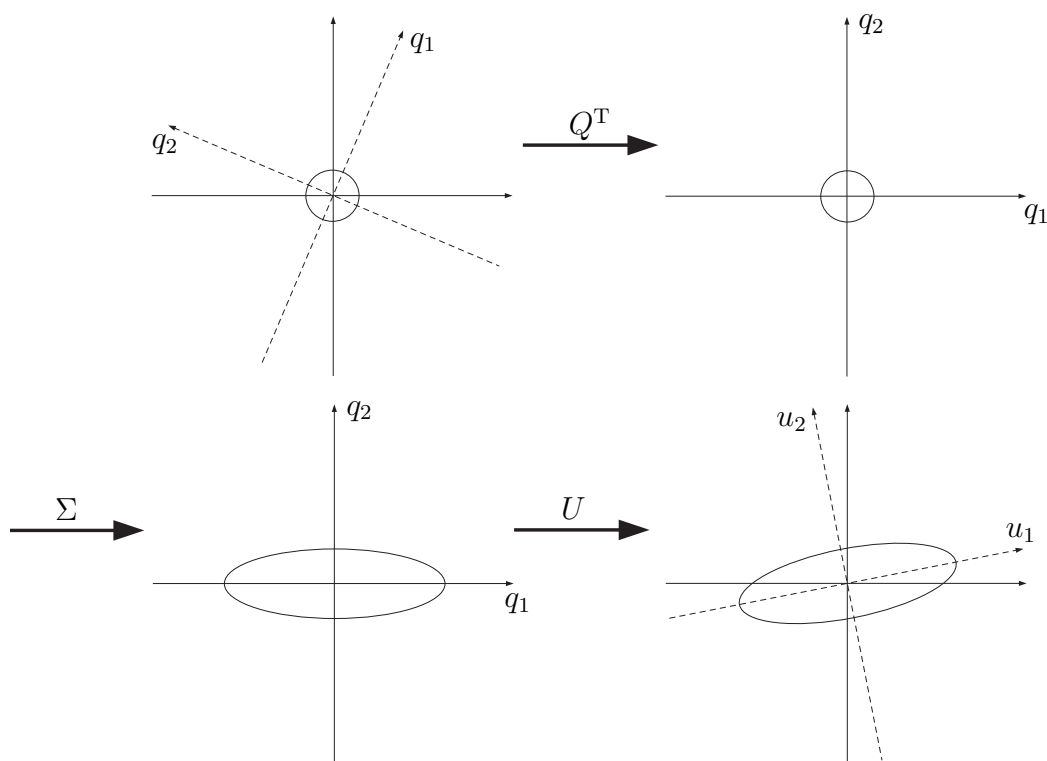
Figure 123: Geometrical interpretation of full SVD [224]: Image of circle \{x \in \mathbb{R}^2 \mid \|x\|_2 = 1\} under matrix multiplication Ax is, in general, an ellipse. For the example illustrated, U \triangleq [u_1 \ u_2] \in \mathbb{R}^{2 \times 2} , Q \triangleq [q_1 \ q_2] \in \mathbb{R}^{2 \times 2} .
