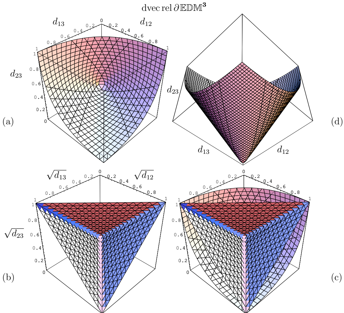
Figure 106: Relative boundary (tiled) of EDM cone \text{EDM}^3 drawn truncated in isometrically isomorphic subspace \mathbb{R}^3 . (a) EDM cone drawn in usual distance-square coordinates d_{ij} . View is from interior toward origin. Unlike positive semidefinite cone, EDM cone is not self-dual, neither is it proper in ambient symmetric subspace (dual EDM cone for this example belongs to isomorphic \mathbb{R}^6 ). (b) Drawn in its natural coordinates \sqrt{d_{ij}} (absolute distance), cone remains convex ( confer §5.10); intersection of three halfspaces (956) whose partial boundaries each contain origin. Cone geometry becomes “complicated” (nonpolyhedral) in higher dimension. [151, §3] (c) Two coordinate systems artificially superimposed. Coordinate transformation from d_{ij} to \sqrt{d_{ij}} appears a topological contraction. (d) Sitting on its vertex \mathbf{0} , pointed \text{EDM}^3 is a circular cone having axis of revolution \text{dvec}(-E) = \text{dvec}(\mathbf{1}\mathbf{1}^T - I) (989) (65). Rounded vertex is plot artifact.
