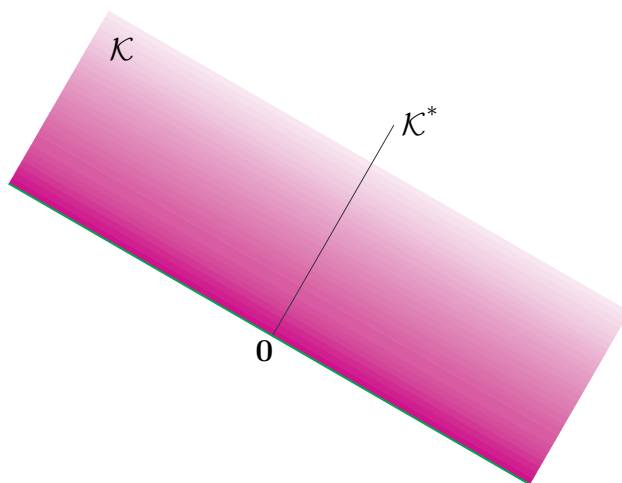
Figure 46: \mathcal{K} is a halfspace about the origin in \mathbb{R}^2 . \mathcal{K}^* is a ray base \mathbf{0} , hence has empty interior in \mathbb{R}^2 ; so \mathcal{K} cannot be pointed. (Both convex cones appear truncated.)
