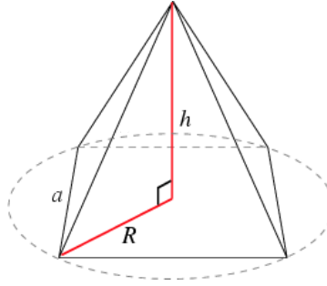
Figure 105: Length of one-dimensional face a equals height h=a=1 of this nonsimplicial pyramid in \mathbb{R}^3 with square base inscribed in a circle of radius R centered at the origin. [315, Pyramid ]
