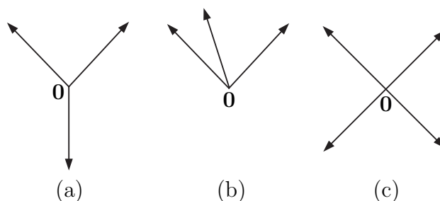
Figure 39: Vectors in \mathbb{R}^2 : (a) affinely and conically independent, (b) affinely independent but not conically independent, (c) conically independent but not affinely independent. None of the examples exhibits linear independence. (In general, a.i. \not\Rightarrow c.i.)
