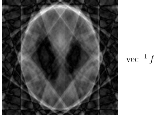
Figure 80: Aliasing of Shepp-Logan phantom in Figure 78 resulting from \mathbf{k} -space subsampling pattern in Figure 79. This image is real because binary mask \Phi is vertically and horizontally symmetric. It is remarkable that the phantom can be reconstructed, by convex iteration, given only \mathcal{U}_0 = \text{vec}^{-1} f .
