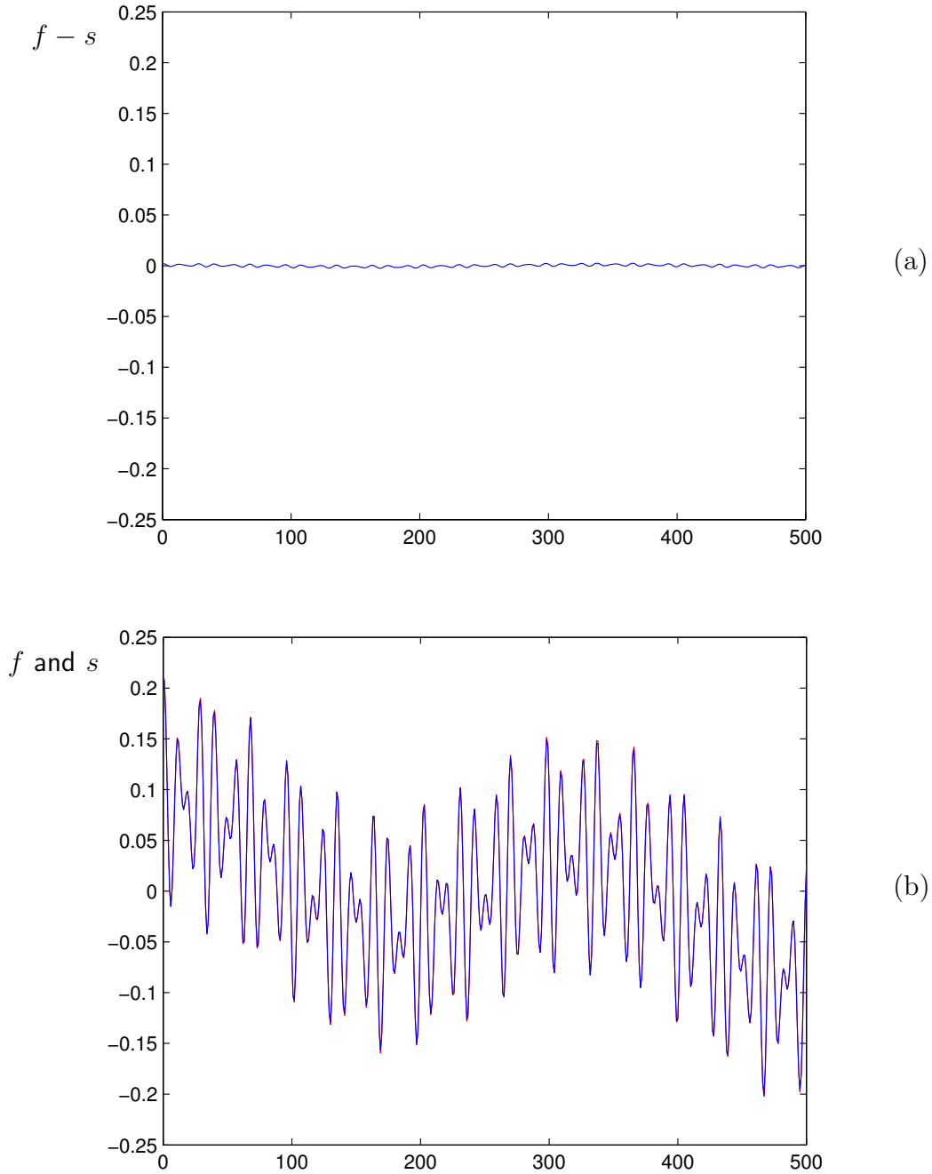
Figure 76: (a) Error signal power (reconstruction f less original noiseless signal s ) is 36dB below s . (b) Original signal s overlaid with reconstruction f (red) from signal g having dropout plus noise.
