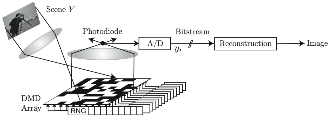
Figure 83: One-pixel camera. [288] [312] Compressive imaging camera block diagram. Incident lightfield (corresponding to the desired image Y ) is reflected off a digital micromirror device (DMD) array whose mirror orientations are modulated in the pseudorandom pattern supplied by the random number generators (RNG). Each different mirror pattern produces a voltage at the single photodiode that corresponds to one measurement y_i .
