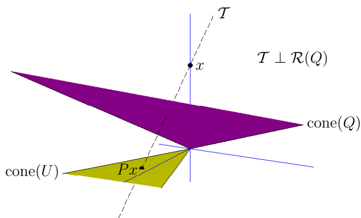
Figure 130: Nonorthogonal projection of x \in \mathbb{R}^3 on \mathcal{R}(U) = \mathbb{R}^2 under biorthogonality condition; id est , Px = UQ^T x such that Q^T U = I . Any point along imaginary line \mathcal{T} connecting x to Px will be projected nonorthogonally on Px with respect to horizontal plane constituting \mathbb{R}^2 = \text{aff cone}(U) in this example. Extreme directions of \text{cone}(U) correspond to two columns of U ; likewise for \text{cone}(Q) . For purpose of illustration, we truncate each conic hull by truncating coefficients of conic combination at unity. Conic hull \text{cone}(Q) is headed upward at an angle, out of plane of page. Nonorthogonal projection would fail were \mathcal{N}(Q^T) in \mathcal{R}(U) (were \mathcal{T} parallel to a line in \mathcal{R}(U) ).
