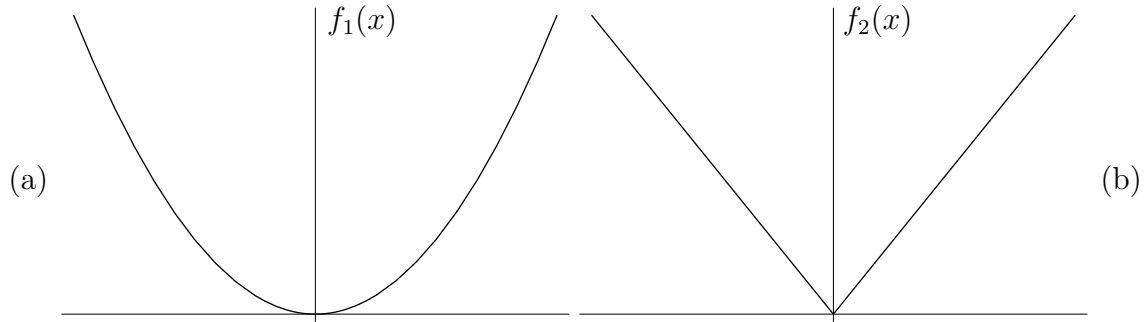
Figure 56: Each convex real function has a unique minimizer x^* but, for x \in \mathbb{R} , f_1(x) = x^2 is strictly convex whereas f_2(x) = \sqrt{x^2} = |x| is not. Strict convexity of a real function is therefore only a sufficient condition for minimizer uniqueness.
