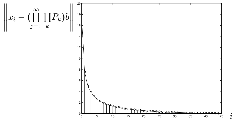
Figure 138: Geometric convergence of iterates in norm, for Example E.10.2.0.2 in \mathbb{R}^{1000} .
