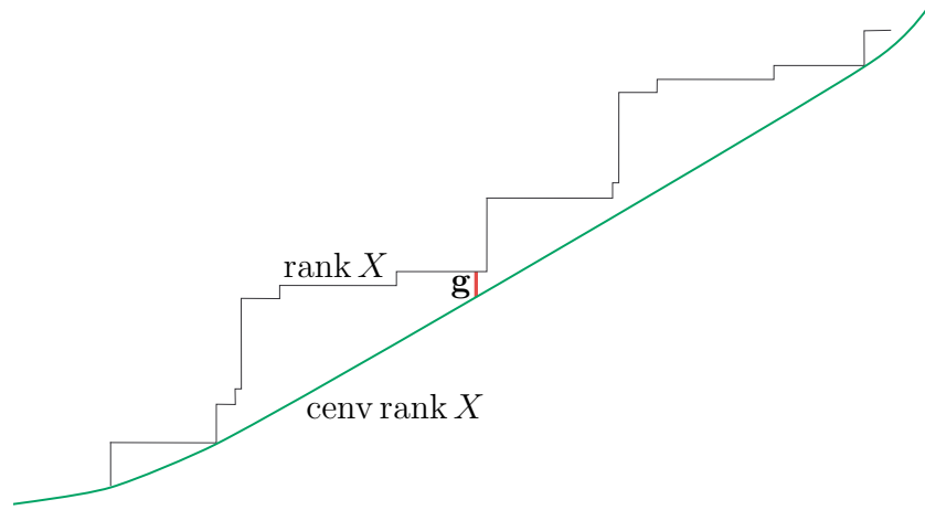
Figure 122: Abstraction of convex envelope of rank function. Rank is a quasiconcave function on the positive semidefinite cone, but its convex envelope is the smallest convex function enveloping it. Vertical bar labelled g illustrates a trace/rank gap; id est , rank found exceeds estimate (by 2).
