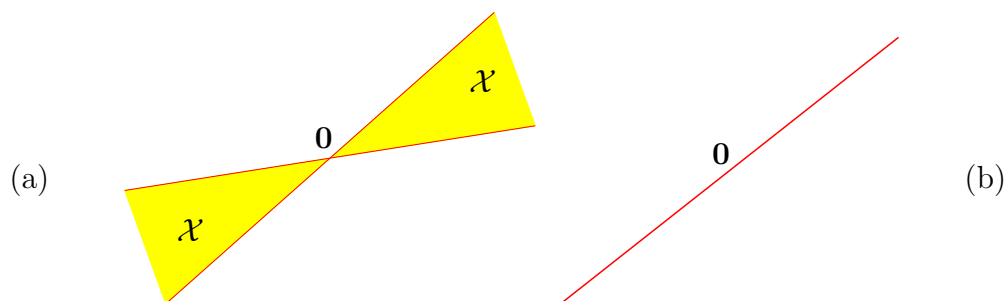
Figure 24: (a) Two-dimensional nonconvex cone drawn truncated. Boundary of this cone is itself a cone. Each polar half is itself a convex cone. (b) This convex cone (drawn truncated) is a line through the origin in any dimension. It has no relative boundary, while its relative interior comprises entire line.
