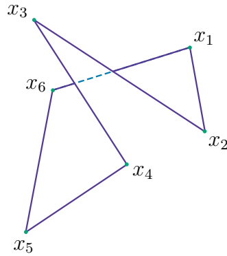
Figure 87: Arbitrary hexagon in \mathbb{R}^3 whose vertices are labelled clockwise.
