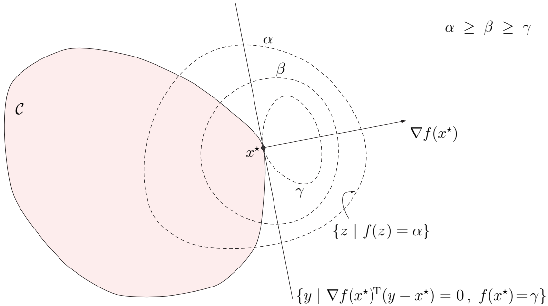
Figure 55: Shown is a plausible contour plot in \mathbb{R}^2 of some arbitrary differentiable real convex function f(x) at selected levels \alpha , \beta , and \gamma ; id est , contours of equal level f (level sets) drawn (dashed) in function's domain. Function is minimized over convex set \mathcal{C} at point x^* iff negative gradient -\nabla f(x^*) belongs to normal cone to \mathcal{C} there. In circumstance depicted, normal cone is a ray whose direction is coincident with negative gradient. From results in §3.1.9 (p.222), \nabla f(x^*) is normal to the \gamma -sublevel set by Definition E.9.1.0.1.
