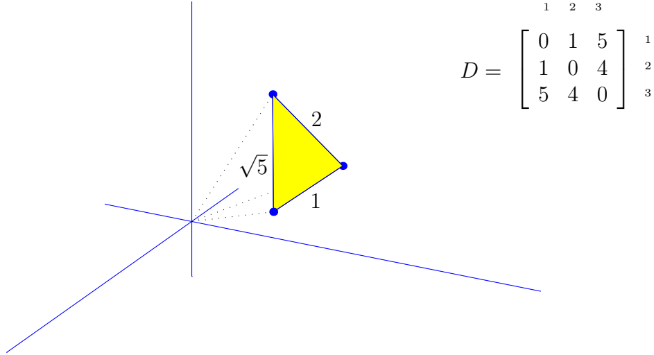
Figure 84: Convex hull of three points ( N = 3 ) is shaded in \mathbb{R}^3 ( n = 3 ). Dotted lines are imagined vectors to points.
