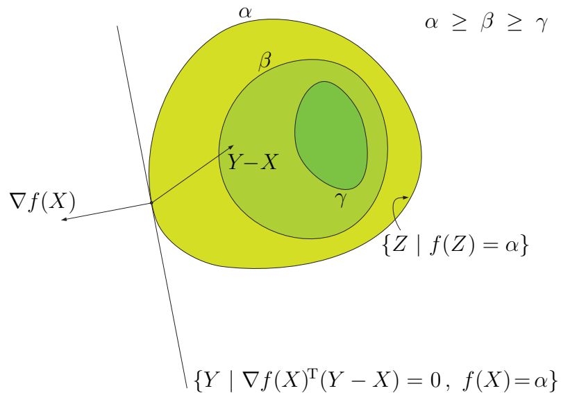
Figure 63: Shown is a plausible contour plot in \mathbb{R}^2 of some arbitrary real convex function f(Z) at selected levels \alpha , \beta , and \gamma ; contours of equal level f (level sets) drawn in the function's domain. A convex function has convex sublevel sets \mathcal{L}_{f(X)}f (540). [255, §4.6] The sublevel set whose boundary is the level set at \alpha , for instance, comprises all the shaded regions. For any particular convex function, the family comprising all its sublevel sets is nested. [165, p.75] Were the sublevel sets not convex, we may certainly conclude the corresponding function is neither convex. Contour plots of real affine functions are illustrated in Figure 19 and Figure 58.
