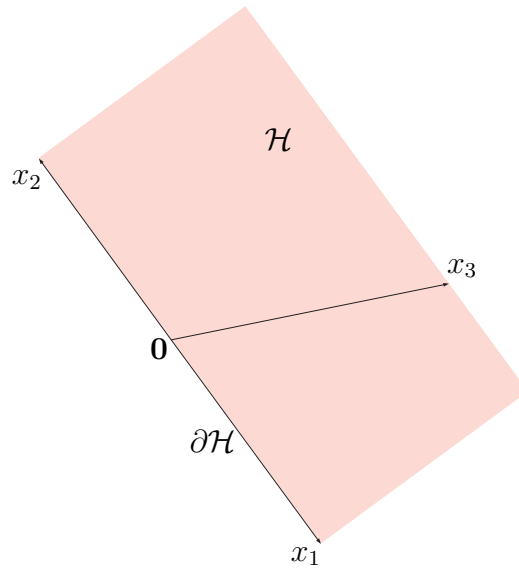
Figure 41: Minimal set of generators X = [x_1 \ x_2 \ x_3] \in \mathbb{R}^{2 \times 3} (not extreme directions) for halfspace about origin; affinely and conically independent.
