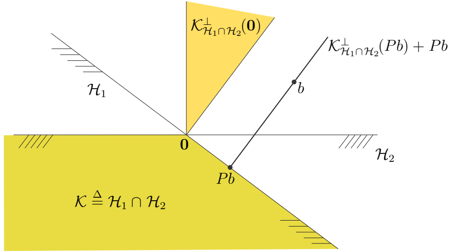
Figure 141: Two examples (truncated): Normal cone to \mathcal{H}_1 \cap \mathcal{H}_2 at the origin, and at point Pb on the boundary. \mathcal{H}_1 and \mathcal{H}_2 are the same halfspaces from Figure 140. The normal cone at the origin \mathcal{K}_{\mathcal{H}_1 \cap \mathcal{H}_2}^\perp(\mathbf{0}) is simply -\mathcal{K}^* .
