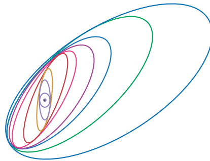
Figure 94: Some fitted contours of equal signal power in \mathbb{R}^2 transmitted from a commercial cellular telephone \bullet over about 1 mile suburban terrain outside San Francisco in 2005. Data courtesy Polaris Wireless. [268]
