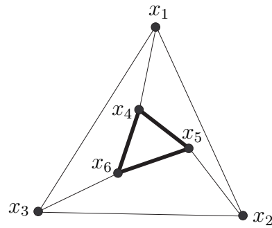
Figure 90: Incomplete EDM corresponding to this dimensionless EDM graph provides unique isometric reconstruction in \mathbb{R}^2 . (drawn freehand, no symmetry intended)
