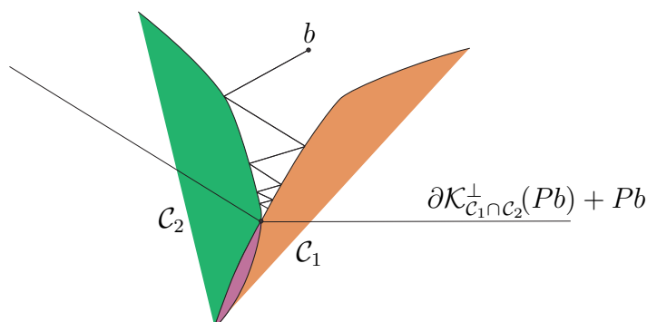
Figure 134: First several alternating projections (1925) in von Neumann-style projection of point b converging on closest point Pb in intersection of two closed convex sets in \mathbb{R}^2 ; C_1 and C_2 are partially drawn in vicinity of their intersection. The pointed normal cone \mathcal{K}^\perp (1954) is translated to Pb , the unique minimum-distance projection of b on intersection. For this particular example, it is possible to start anywhere in a large neighborhood of b and still converge to Pb . The alternating projections are themselves robust with respect to some significant amount of noise because they belong to translated normal cone.
