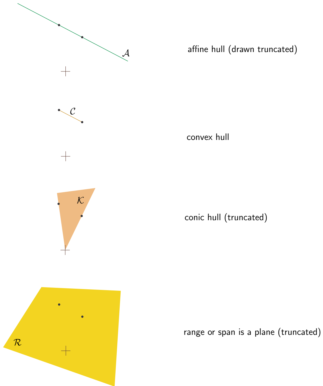
Figure 15: Given two points in Euclidean vector space of any dimension, their various hulls are illustrated. Each hull is a subset of range; generally, \mathcal{A}, \mathcal{C}, \mathcal{K} \subseteq \mathcal{R} . (Cartesian axes drawn for reference.)
