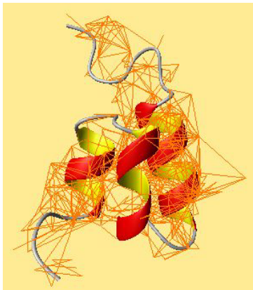
Figure 3: [154] [94] Distance data collected via nuclear magnetic resonance (NMR) helped render this 3-dimensional depiction of a protein molecule. At the beginning of the 1980s, Kurt Wüthrich [Nobel laureate] developed an idea about how NMR could be extended to cover biological molecules such as proteins. He invented a systematic method of pairing each NMR signal with the right hydrogen nucleus (proton) in the macromolecule. The method is called sequential assignment and is today a cornerstone of all NMR structural investigations. He also showed how it was subsequently possible to determine pairwise distances between a large number of hydrogen nuclei and use this information with a mathematical method based on distance-geometry to calculate a three-dimensional structure for the molecule. –[232] [319] [149]
