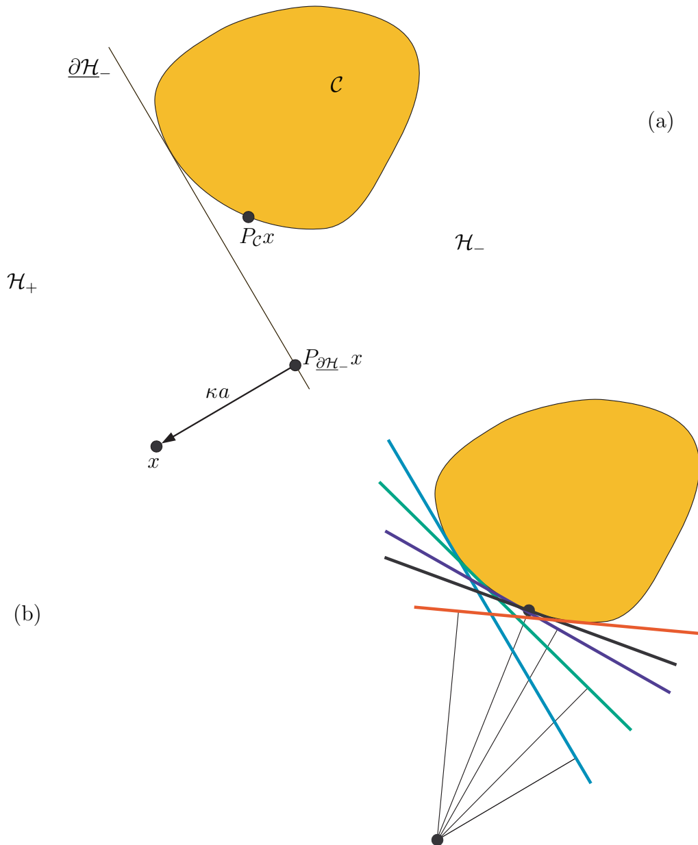
Figure 132: Dual interpretation of projection of point x on convex set \mathcal{C} in \mathbb{R}^2 . (a) \kappa = (a^T a)^{-1} (a^T x - \sigma_{\mathcal{C}}(a)) (b) Minimum distance from x to \mathcal{C} is found by maximizing distance to all hyperplanes supporting \mathcal{C} and separating it from x . A convex problem for any convex set, distance of maximization is unique.
