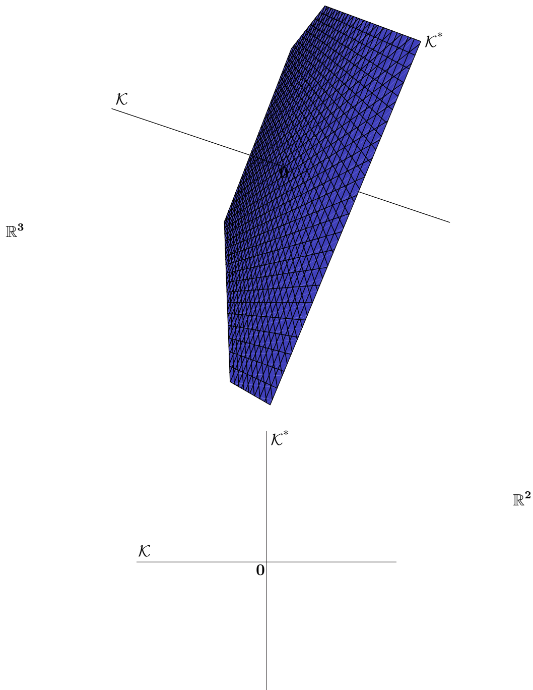
Figure 48: When convex cone \mathcal{K} is any one Cartesian axis, its dual cone is the convex hull of all axes remaining. In \mathbb{R}^3 , dual cone \mathcal{K}^* (drawn tiled and truncated) is a hyperplane through origin; its normal belongs to line \mathcal{K} . In \mathbb{R}^2 , dual cone \mathcal{K}^* is a line through origin while convex cone \mathcal{K} is that line orthogonal.
