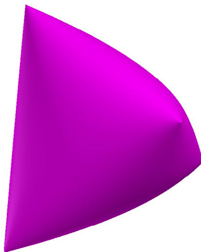
Figure 98: Elliptope \mathcal{E}^3 in isometrically isomorphic \mathbb{R}^6 (projected on \mathbb{R}^3 ) is a convex body that appears to possess some kind of symmetry in this dimension; it resembles a malformed pillow in the shape of a bulging tetrahedron. Elliptope relative boundary is not smooth and comprises all set members (970) having at least one 0 eigenvalue. [195, §2.1] This elliptope has an infinity of vertices, but there are only four vertices corresponding to a rank-1 matrix. Those yy^T , evident in the illustration, have binary vector y \in \mathbb{R}^3 with entries in \{\pm 1\} .
