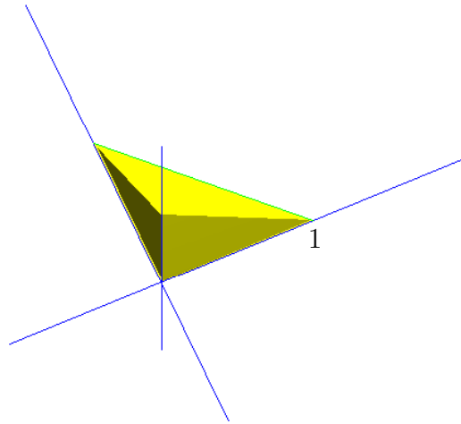
Figure 42: Unit simplex \mathcal{S} in \mathbb{R}^3 is a unique solid tetrahedron, but is not regular .
