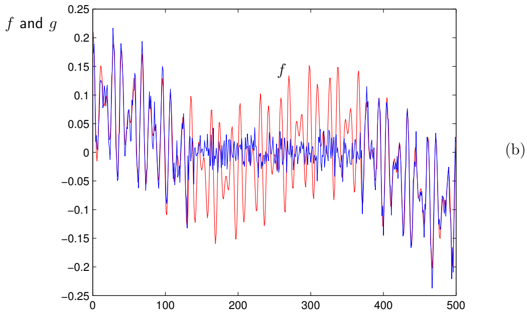
Figure 75: (a) Signal dropout in signal s corrupted by noise \eta (SNR = 10dB, g = s + \eta ). Flatline indicates duration of signal dropout. (b) Reconstructed signal f (red) overlaid with corrupted signal g .
