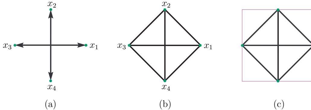
Figure 96: (a) Four points in quadrature in two dimensions about their geometric center. (b) Complete EDM graph of diamond vertices. (c) Quadrature rotation of a Euclidean body in \mathbb{R}^2 first requires a shroud that is the smallest Cartesian square containing it.
