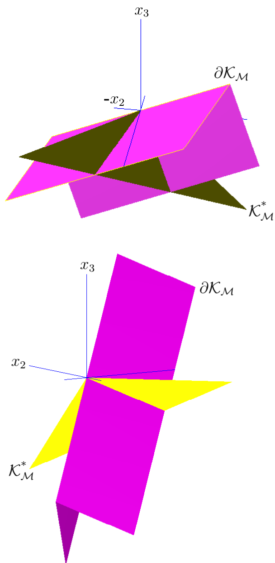
Figure 54: Two views of monotone cone \mathcal{K}_{\mathcal{M}} and its dual \mathcal{K}_{\mathcal{M}}^* (drawn truncated) in \mathbb{R}^3 . Monotone cone is not pointed. Dual monotone cone has empty interior. Cartesian coordinate axes are drawn for reference.
