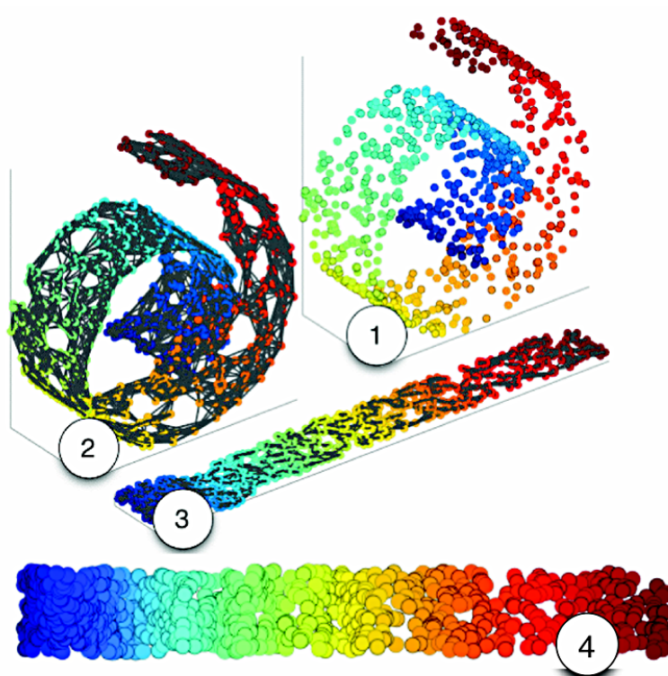
Figure 5: Swiss roll from Weinberger & Saul [314]. The problem of manifold learning, illustrated for N = 800 data points sampled from a “Swiss roll” ①. A discretized manifold is revealed by connecting each data point and its k = 6 nearest neighbors ②. An unsupervised learning algorithm unfolds the Swiss roll while preserving the local geometry of nearby data points ③. Finally, the data points are projected onto the two dimensional subspace that maximizes their variance, yielding a faithful embedding of the original manifold ④.
