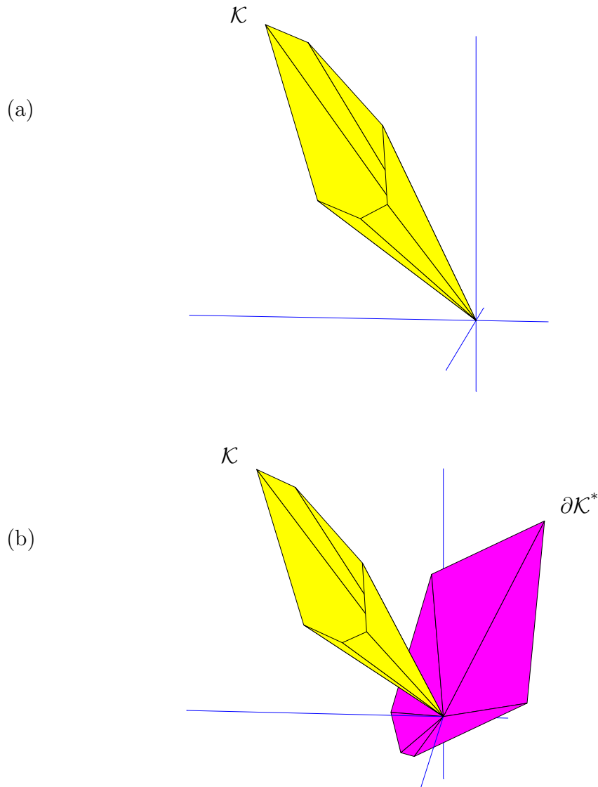
Figure 40: (a) A pointed polyhedral cone (drawn truncated) in \mathbb{R}^3 having six facets. The extreme directions, corresponding to six edges emanating from the origin, are generators for this cone; not linearly independent but they must be conically independent. (b) The boundary of dual cone \mathcal{K}^* (drawn truncated) is now added to the drawing of same \mathcal{K} . \mathcal{K}^* is polyhedral, proper, and has the same number of extreme directions as \mathcal{K} has facets.
