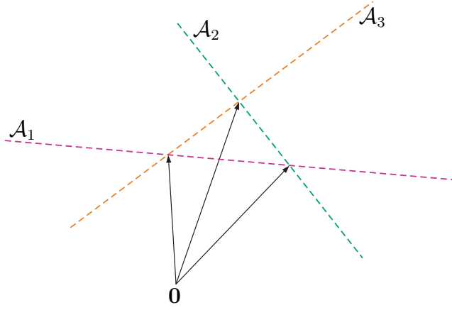
Figure 20: Any one particular point of three points illustrated does not belong to affine hull \mathcal{A}_i ( i \in 1, 2, 3 , each drawn truncated) of points remaining. Three corresponding vectors in \mathbb{R}^2 are, therefore, affinely independent (but neither linearly or conically independent).
