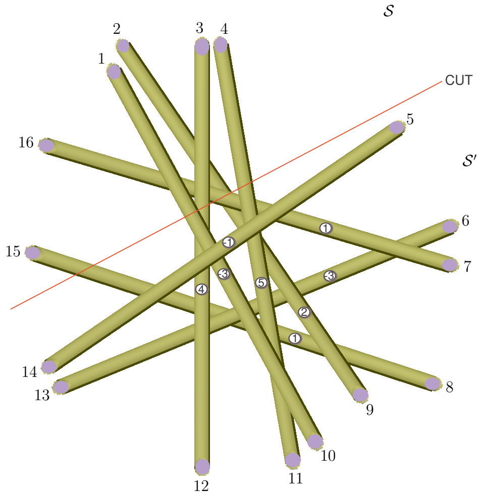
Figure 77: A CUT partitions nodes \{i=1 \dots 16\} of this graph into \mathcal{S} and \mathcal{S}' . Linear arcs have circled weights. The problem is to find a cut maximizing total weight of all arcs linking partitions made by the cut.
