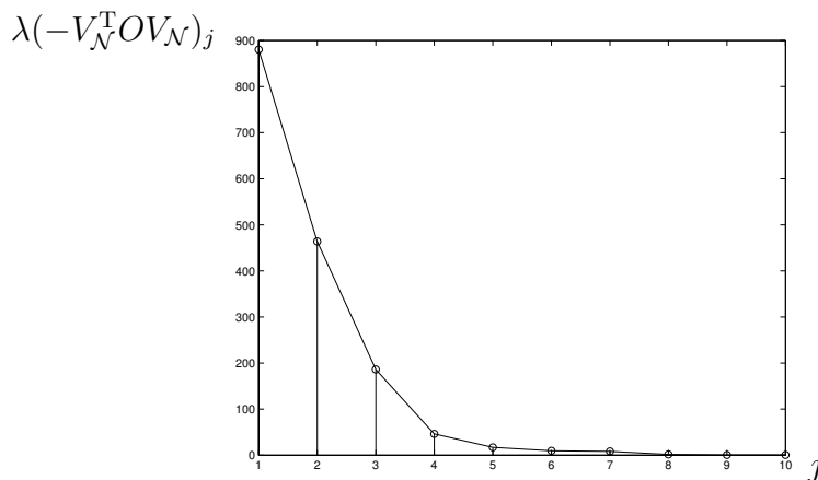
Figure 103: Largest ten eigenvalues of -V_N^T O V_N for map of USA, sorted by nonincreasing value. In the code (§F), we normalize O by (N(N-1)/2)^2 .
