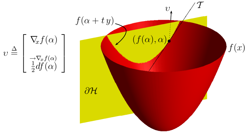
Figure 128: Convex quadratic bowl in \mathbb{R}^2 \times \mathbb{R} ; f(x) = x^T x : \mathbb{R}^2 \rightarrow \mathbb{R} versus x on some open disc in \mathbb{R}^2 . Plane slice \partial\mathcal{H} is perpendicular to function domain. Slice intersection with domain connotes bidirectional vector y . Slope of tangent line \mathcal{T} at point (\alpha, f(\alpha)) is value of directional derivative \nabla_x f(\alpha)^T y (1701) at \alpha in slice direction y . Negative gradient -\nabla_x f(x) \in \mathbb{R}^2 is direction of steepest descent . [316] [180, §15.6] [121] When vector v \in \mathbb{R}^3 entry v_3 is half directional derivative in gradient direction at \alpha and when \begin{bmatrix} v_1 \\ v_2 \end{bmatrix} = \nabla_x f(\alpha) , then -v points directly toward bowl bottom.
