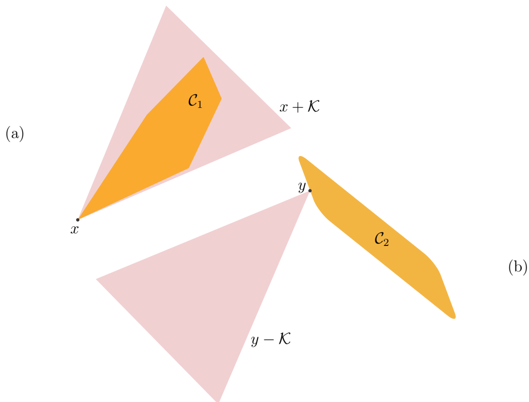
Figure 30: (a) Point x is the minimum element of set \mathcal{C}_1 with respect to cone \mathcal{K} because cone translated to x \in \mathcal{C}_1 contains set. (b) Point y is a minimal element of set \mathcal{C}_2 with respect to cone \mathcal{K} because negative cone translated to y \in \mathcal{C}_2 contains only y . (Cones drawn truncated in \mathbb{R}^2 .)
