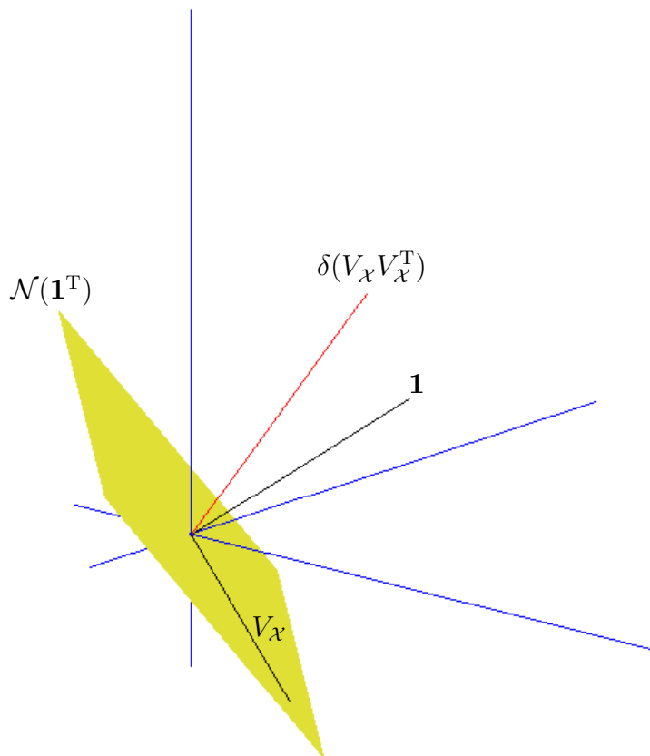
Figure 111: Example of V_{\mathcal{X}} selection to make an EDM corresponding to cardinality N=3 and affine dimension r=1 ; V_{\mathcal{X}} is a vector in nullspace \mathcal{N}(\mathbf{1}^T) \subset \mathbb{R}^3 . Nullspace of \mathbf{1}^T is hyperplane in \mathbb{R}^3 (drawn truncated) having normal \mathbf{1} . Vector \delta(V_{\mathcal{X}}V_{\mathcal{X}}^T) may or may not be in plane spanned by \{\mathbf{1}, V_{\mathcal{X}}\} , but belongs to nonnegative orthant which is strictly supported by \mathcal{N}(\mathbf{1}^T) .
