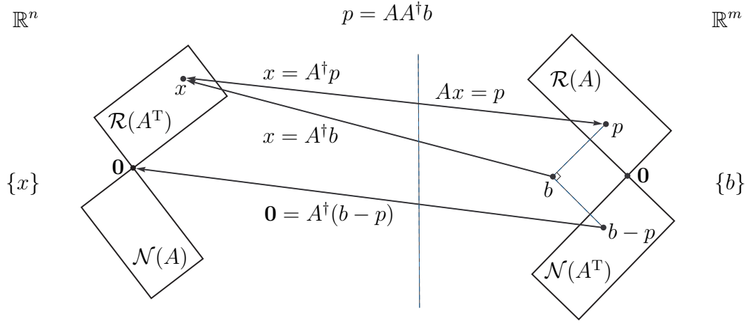
Figure 129: Action of pseudoinverse A^\dagger \in \mathbb{R}^{n \times m} : [277, p.449] Component of vector b in \mathcal{N}(A^T) maps to origin, while component of b in \mathcal{R}(A) maps to row space \mathcal{R}(A^T) . For any A \in \mathbb{R}^{m \times n} , inversion is bijective \forall p \in \mathcal{R}(A) .
