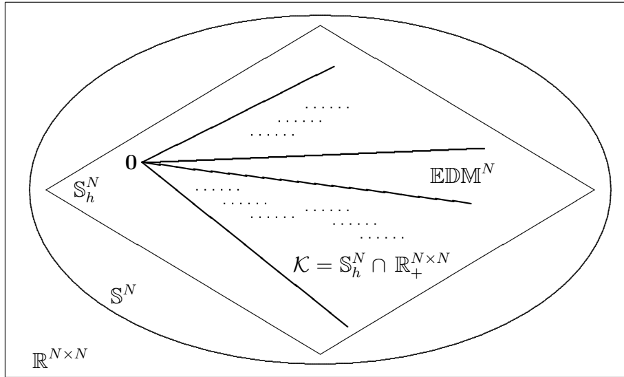
Figure 120: Pseudo-Venn diagram: The EDM cone belongs to the intersection of the symmetric hollow subspace with the nonnegative orthant; \mathbb{EDM}^N \subseteq \mathcal{K} (786). \mathbb{EDM}^N cannot exist outside \mathbb{S}_h^N , but \mathbb{R}_+^{N \times N} does.
