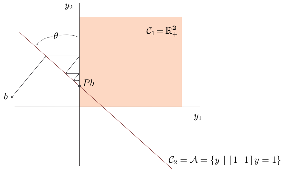
Figure 137: From Example E.10.2.0.2 in \mathbb{R}^2 , showing von Neumann-style alternating projection to find feasible point belonging to intersection of nonnegative orthant with hyperplane. Point Pb lies at intersection of hyperplane with ordinate axis. In this particular example, the feasible point found is coincidentally optimal. Rate of convergence depends upon angle \theta ; as it becomes more acute, convergence slows. [142, §3]
