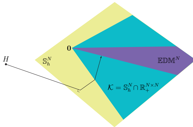
Figure 121: Pseudo-Venn diagram from Figure 120 showing elbow placed in path of projection of H on \text{EDM}^N \subset S_h^N by an optimization problem demanding nonnegative input matrix H . The first two line segments leading away from H result from correct order-of-projection required to provide nonnegative H prior to optimization. Were H nonnegative, then its projection on S_h^N would instead belong to \mathcal{K} ; making the elbow disappear. (confer Figure 133)
