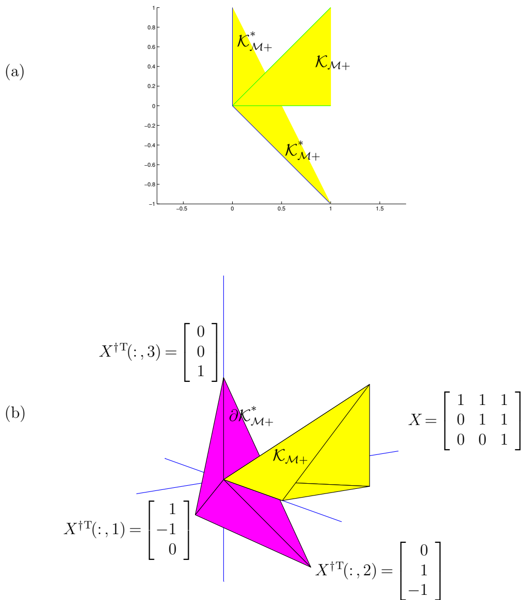
Figure 52: Simplicial cones. (a) Monotone nonnegative cone \mathcal{K}_{\mathcal{M}+} and its dual \mathcal{K}_{\mathcal{M}+}^* (drawn truncated) in \mathbb{R}^2 . (b) Monotone nonnegative cone and boundary of its dual (both drawn truncated) in \mathbb{R}^3 . Extreme directions of \mathcal{K}_{\mathcal{M}+}^* are indicated.
