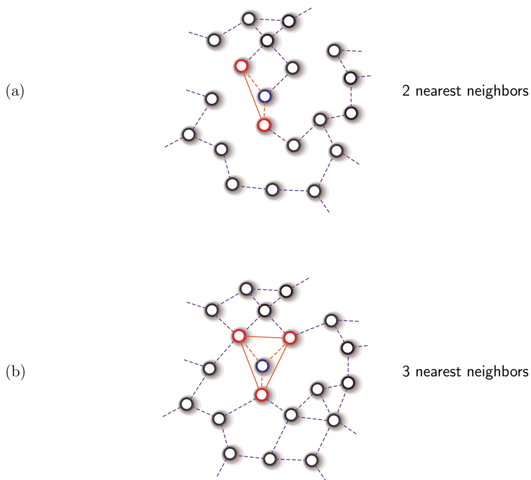
Figure 108: Neighborhood graph (dashed) with dimensionless EDM subgraph completion (solid) superimposed (but not covering dashed). Local view of a few dense samples \circ from relative interior of some arbitrary Euclidean manifold whose affine dimension appears two-dimensional in this neighborhood. All line segments measure absolute distance. Dashed line segments help visually locate nearest neighbors; suggesting, best number of nearest neighbors can be greater than value of embedding dimension after topological transformation. ( confer [174, §2]) Solid line segments represent completion of EDM subgraph from available distance data for an arbitrarily chosen sample and its nearest neighbors. Each distance from EDM subgraph becomes distance-square in corresponding EDM submatrix.
