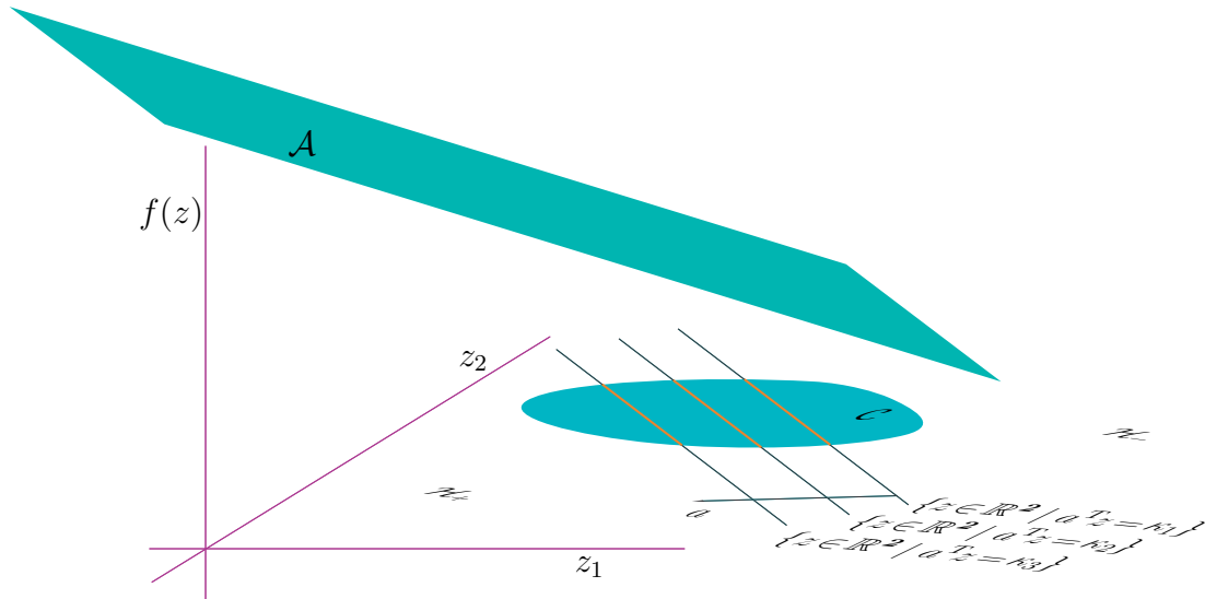
Figure 58: Cartesian axes in \mathbb{R}^3 and three hyperplanes intersecting convex set C \subset \mathbb{R}^2 reproduced from Figure 21. Plotted with third dimension is affine set \mathcal{A} = f(\mathbb{R}^2) a plane. Sequence of hyperplanes, w.r.t domain \mathbb{R}^2 of an affine function f(z) = a^T z + b : \mathbb{R}^2 \rightarrow \mathbb{R} , is increasing in direction of gradient a (§3.1.8.0.3) because affine function increases in normal direction (Figure 19).
