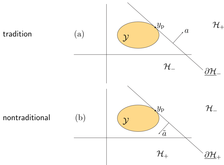
Figure 22: (a) Hyperplane \underline{\partial\mathcal{H}}_- (116) supporting closed set \mathcal{Y} \in \mathbb{R}^2 . Vector a is inward-normal to hyperplane with respect to halfspace \mathcal{H}_+ , but outward-normal with respect to set \mathcal{Y} . A supporting hyperplane can be considered the limit of an increasing sequence in the normal-direction like that in Figure 21. (b) Hyperplane \underline{\partial\mathcal{H}}_+ nontraditionally supporting \mathcal{Y} . Vector \tilde{a} is inward-normal to hyperplane now with respect to both halfspace \mathcal{H}_+ and set \mathcal{Y} . Tradition [165] [255] recognizes only positive normal polarity in support function \sigma_{\mathcal{Y}} as in (117); id est , normal a , figure (a). But both interpretations of supporting hyperplane are useful.
