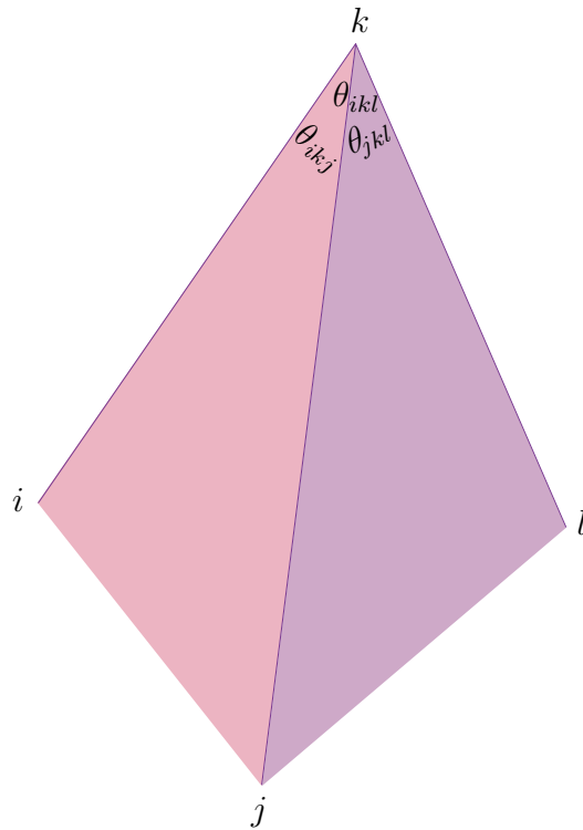
Figure 86: Nomenclature for fifth Euclidean metric property. Each angle \theta is made by a vector pair at vertex k while i, j, k, l index four points. The fifth property is necessary for realization of four or more points; a reckoning by three angles in any dimension.
