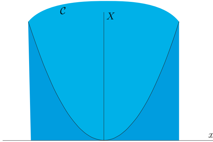
Figure 34: Convex set \mathcal{C} = \{X \in \mathbb{S} \times x \in \mathbb{R} \mid X \succeq xx^T\} drawn truncated.
