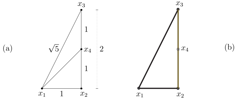
Figure 85: (a) Complete dimensionless EDM graph . (b) Emphasizing obscured segments \overline{x_2x_4} , \overline{x_4x_3} , and \overline{x_2x_3} , now only five (2N - 3) absolute distances are specified. EDM so represented is incomplete, missing d_{14} as in (779), yet the isometric reconstruction (§5.4.2.2.6) is unique as proved in §5.9.3.0.1 and §5.14.4.1.1. First four properties of Euclidean metric are not a recipe for reconstruction of this polyhedron.
