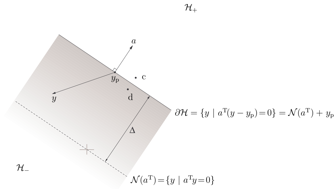
Figure 18: Hyperplane illustrated \partial\mathcal{H} is a line partially bounding halfspaces \mathcal{H}_- = \{y \mid a^T(y - y_p) \leq 0\} and \mathcal{H}_+ = \{y \mid a^T(y - y_p) \geq 0\} in \mathbb{R}^2 . Shaded is a rectangular piece of semi-infinite \mathcal{H}_- with respect to which vector a is outward-normal to bounding hyperplane; vector a is inward-normal with respect to \mathcal{H}_+ . Halfspace \mathcal{H}_- contains nullspace \mathcal{N}(a^T) (dashed line through origin) because a^T y_p > 0 . Hyperplane, halfspace, and nullspace are each drawn truncated. Points c and d are equidistant from hyperplane, and vector c - d is normal to it. \Delta is distance from origin to hyperplane.
