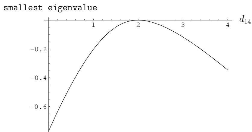
Figure 100: Smallest eigenvalue of -V_{\mathcal{N}}^T D V_{\mathcal{N}} makes it a PSD matrix for only one value of d_{14} : 2.
