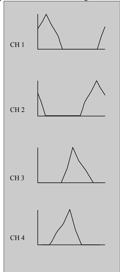
Figure 6. Control functions for angular displacement, CH 1 - CH 4 .
