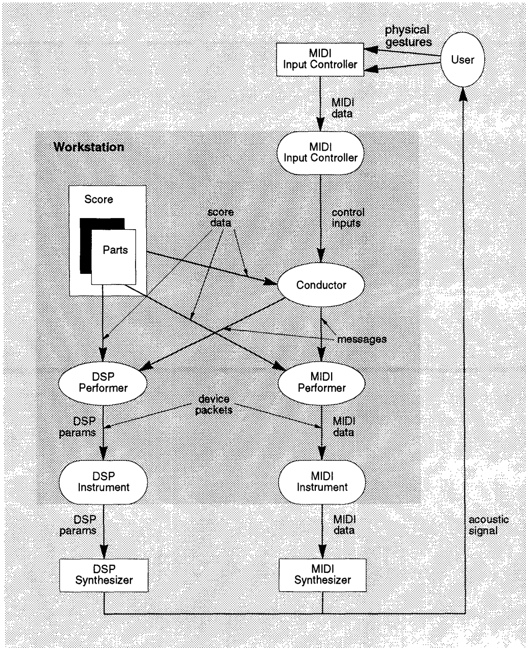
FIGURE 4.4 ZED objects and data flow.
