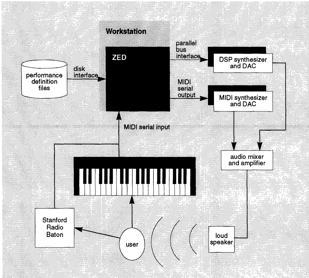
FIGURE 4.1 ZED real-time music performance workstation.
