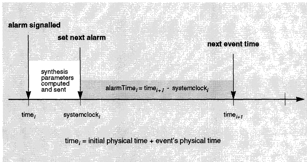
FIGURE 6.4 Real-time performance execution loop.
