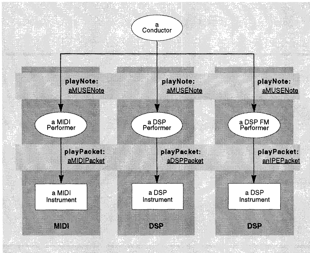
FIGURE 4.6 Performer and instrument interfaces.
