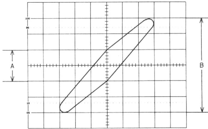
Fig. 2-9. DUAL-TRACE METHOD OF PHASE MEASUREMENT
