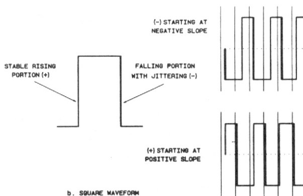
Fig. 2-4. TRIGGER POINT SELECTION
