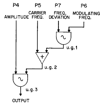
Fig. 9. Simple FM circuit as represented in MUSIC V notation.
