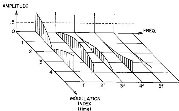
Fig. 7. Dynamic spectrum where the ratio c/m = 1/1 and the modulation index increases from 0 to 4 continuously. The increasing bandwidth is easily seen, but because the spectrum includes the reflected side frequencies, the evolution of the individual components is not always intuitively clear.
