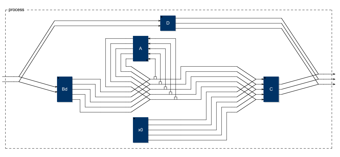
Figure 20: State-space model in FAUST having 2 inputs, 3 outputs, and 5 state variables.
