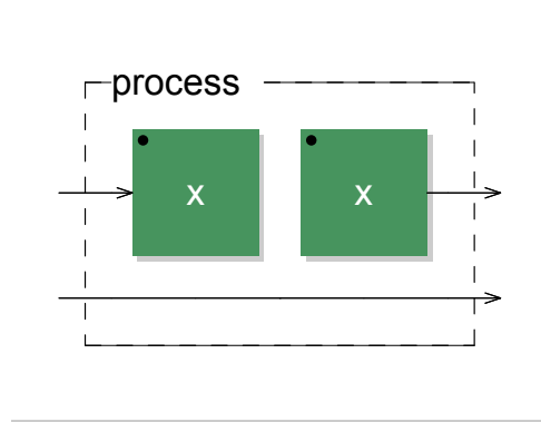
Figure 4: process(x) = x,-;
