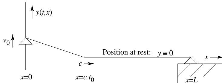
Moving rigid termination for an ideal string.
