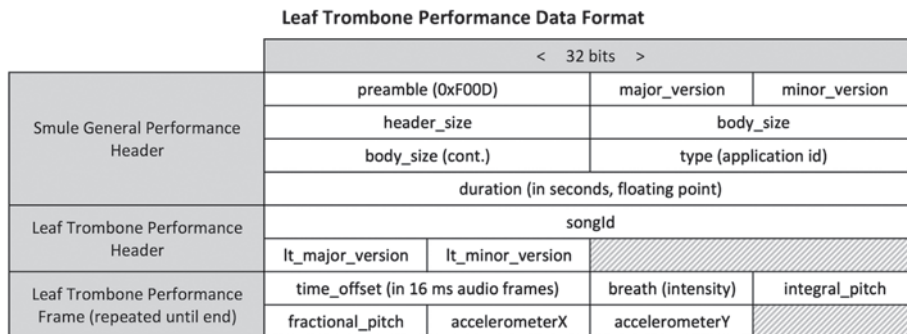
Fig. 10. The data format for a Leaf Trombone: World Stage performance. Each row represents 4 bytes (32 bits), with 1-, 2-, or 4-byte subdivisions thereof for individual data fields.
