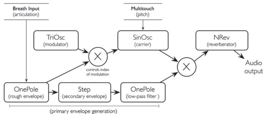
Fig. 4. ChuckK block diagram for synthesizing the Leaf Trombone. In the two-operator FM setup, both the carrier oscillator and modulator oscillator are enveloped by breath input, thereby increasing the spectral brightness with the instrument's attack and creating a distinctively brass-like tone.
