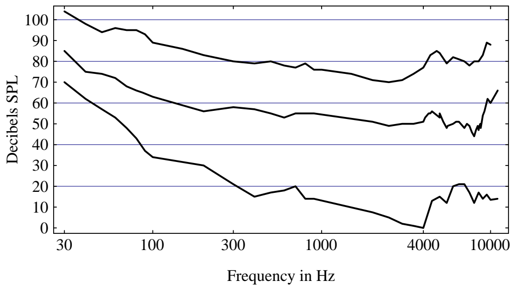
Fletcher-Munson Curve of Equal Loudness
