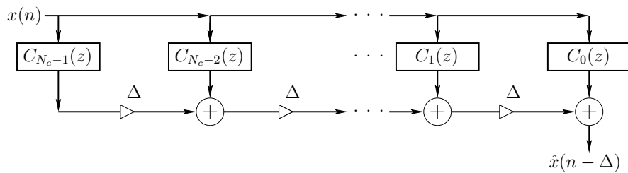
Farrow Structure
