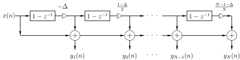
Truncated Taylor Expansion
