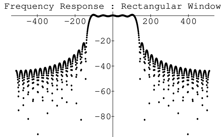
Truncated-Sinc Transform
