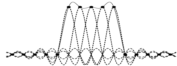
Bandlimited Rectangular Pulse Reconstruction from its Samples
